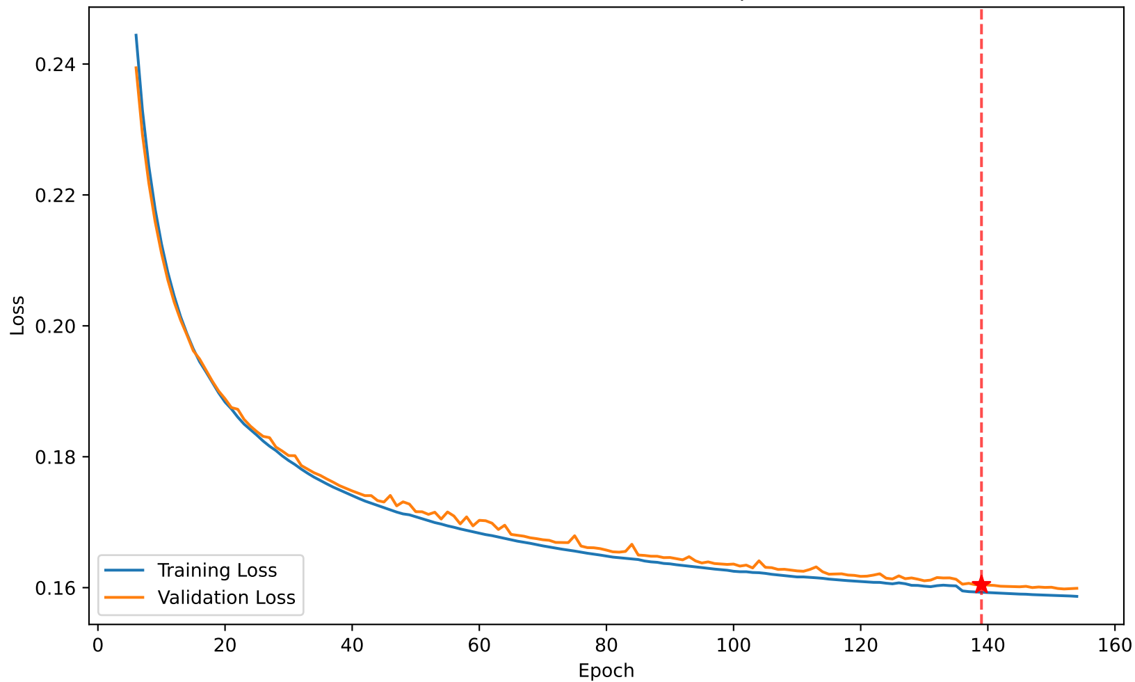
Loss 0.159 vs Val Loss 0.160 at epoch 139
