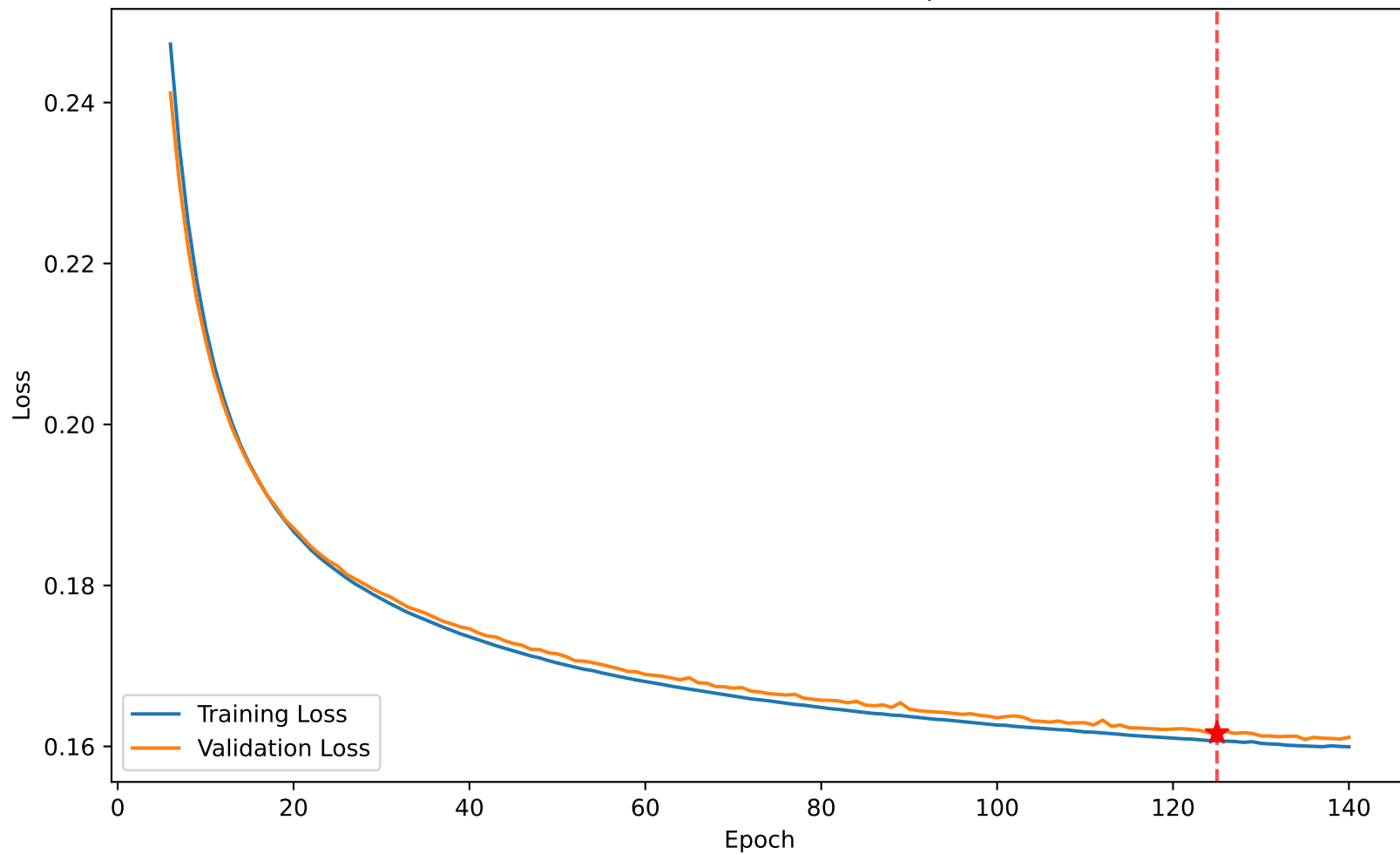
Loss 0.161 vs Val Loss 0.162 at epoch 125
