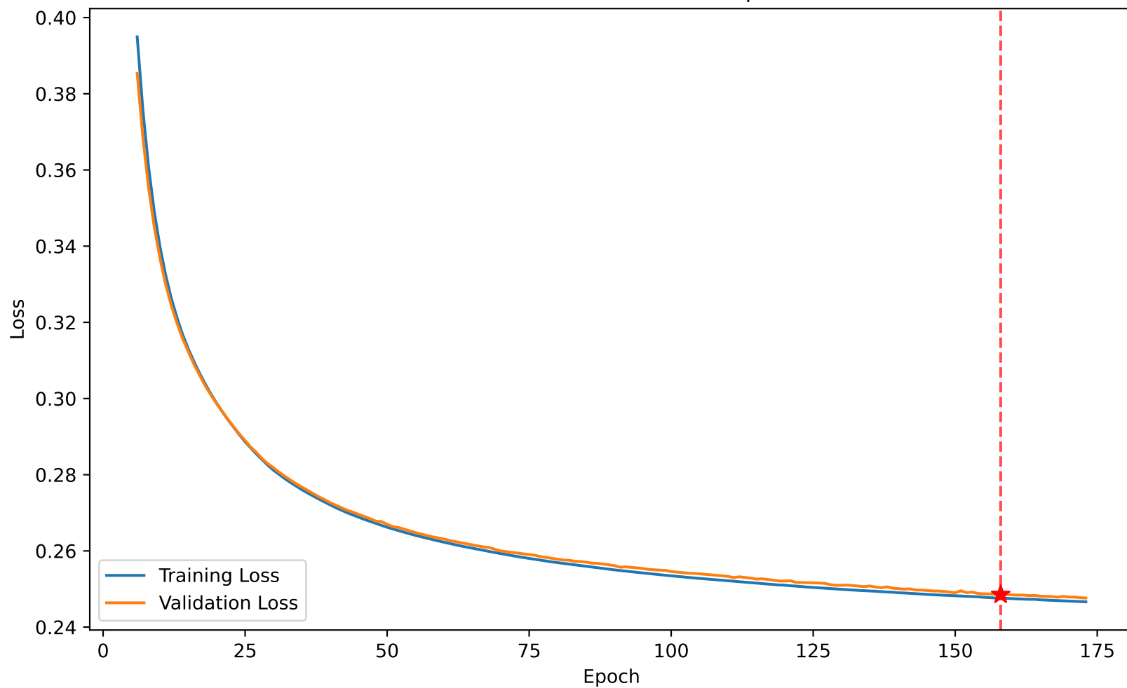
Loss 0.248 vs Val Loss 0.249 at epoch 158
