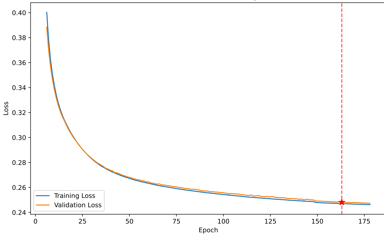
Loss 0.247 vs Val Loss 0.248 at epoch 163
