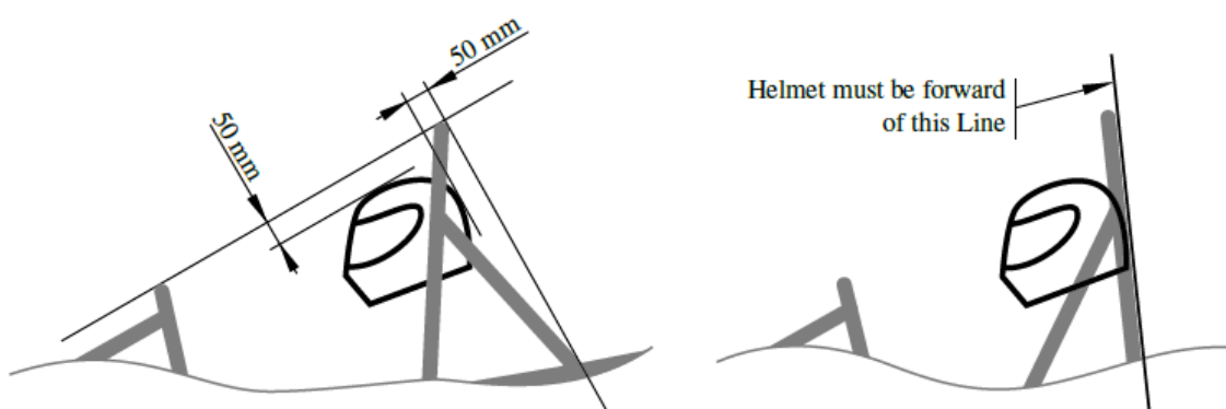
Figure13: Minimum helmet clearance
