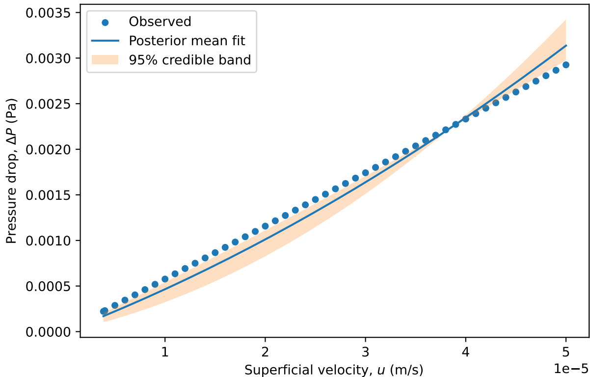
Pressure-drop fit: Medium pumice stones
