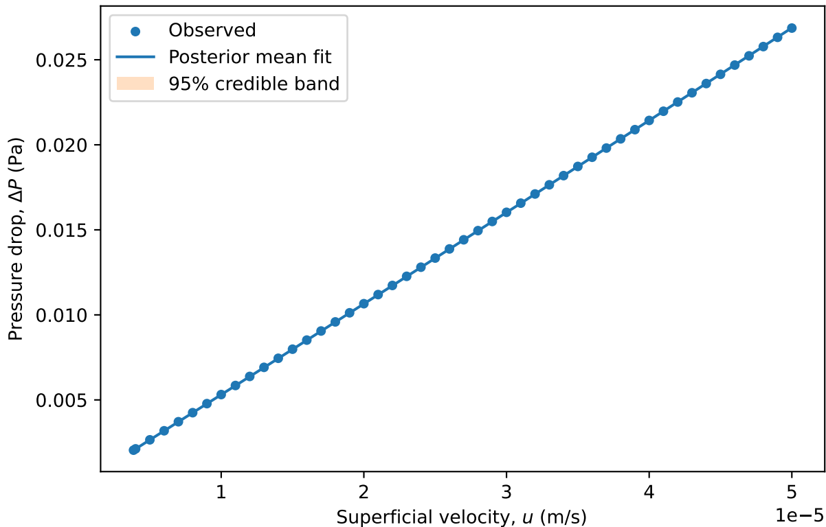
Pressure-drop fit: Glass marbles
