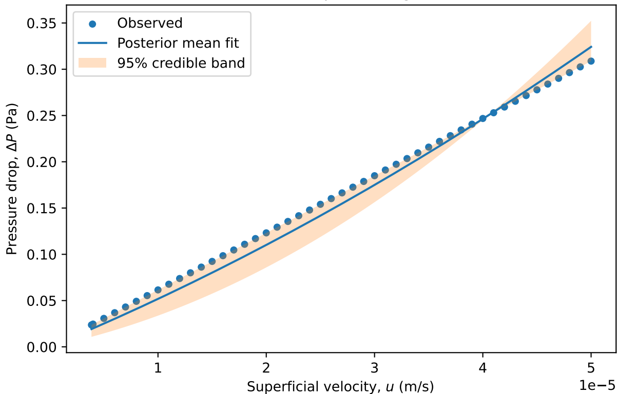
Pressure-drop fit: Pea gravels
