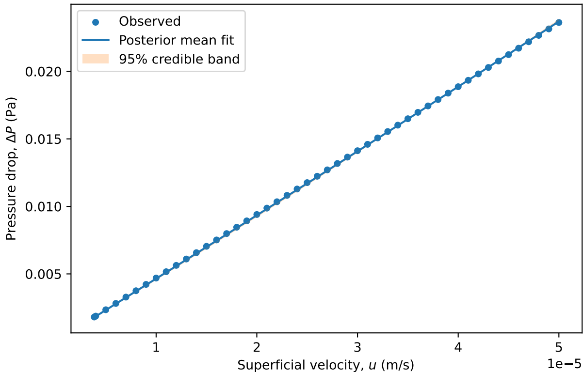
Pressure-drop fit: Small pumice stones
