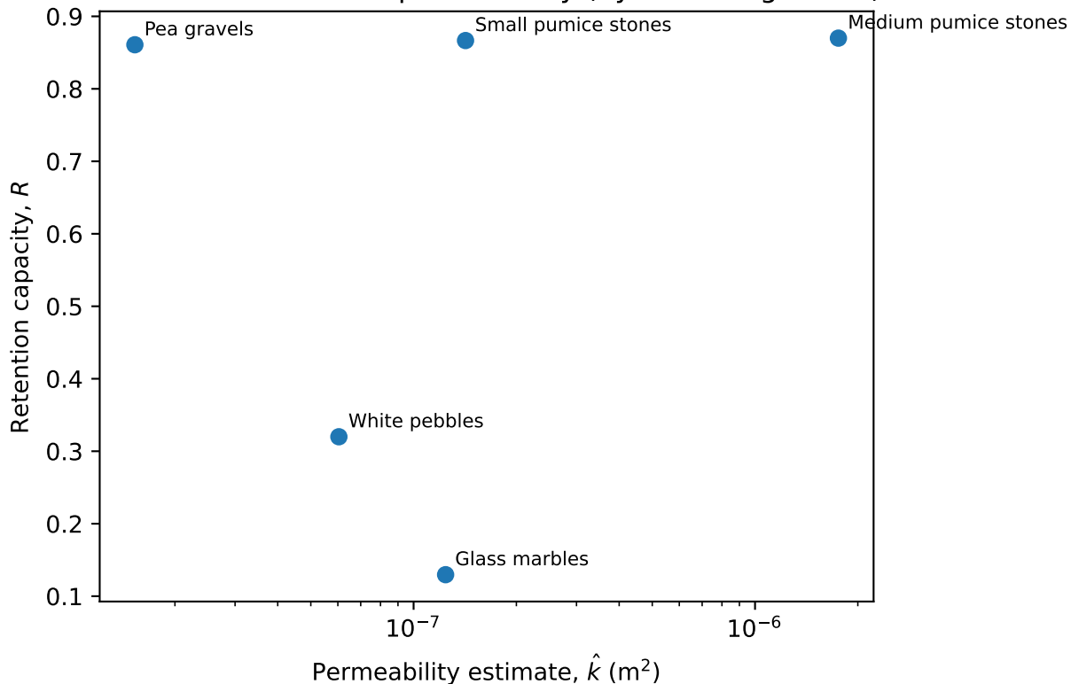
Retention vs inferred permeability (hydraulic signature)
