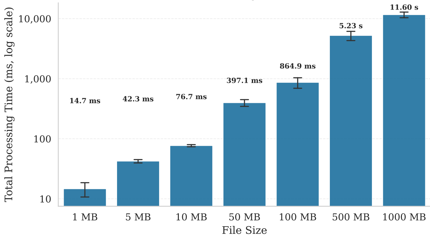
End-to-End Processing Time vs. File Size
