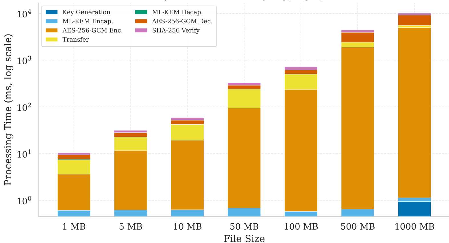
Processing Time Breakdown by Cryptographic Phase
