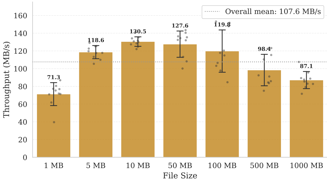
End-to-End Throughput vs. File Size
