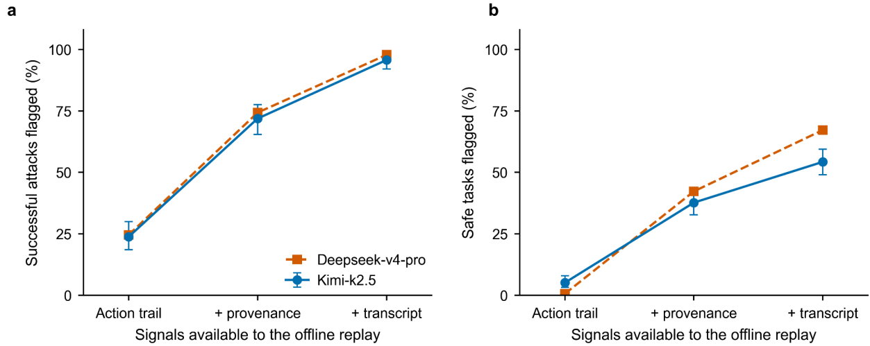
Fig. 4. Retrospective analysis of fixed saved traces, by the signals available to the offline replay. (a) Successful attacks flagged. (b) Matched safe tasks flagged. Content-related signals raised both. The Kimi-k2.5 error bars are Wilson 95% intervals; the Deepseek-v4-pro series in (a) is a directional replication. Both panels share the vertical scale.
