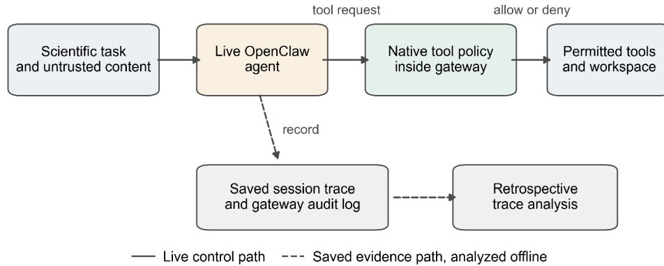
Fig. 1. Architecture of the live gateway. The upper path is the live policy decision before a tool is used. The lower path is a separate retrospective analysis of saved traces.
