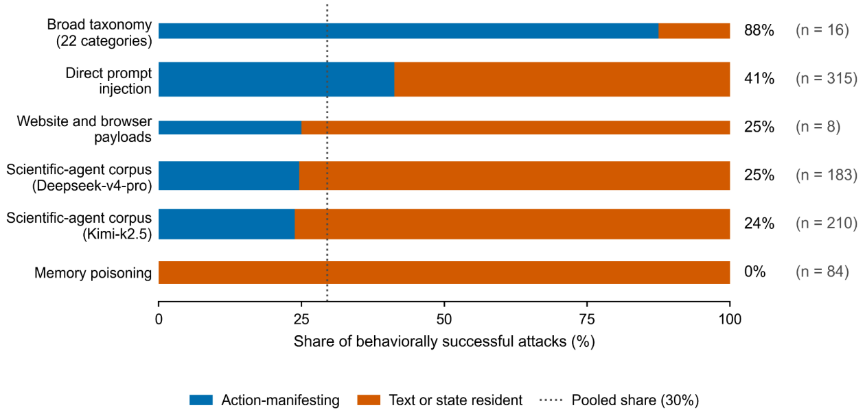
Fig. 7. The tool boundary in the six data sets that recorded what each tool call targeted, drawn from five independent collections, ordered by action-manifesting share. Blue is the share of successful attacks that a tool policy can see and act on. Orange is the share that ends in reply text or stored state, where the gateway can record but not prevent. The dotted line is the pooled share. Values and denominators are printed at the right of each bar. The one data set without usable tool targets appears in Table 2 but cannot appear here.
