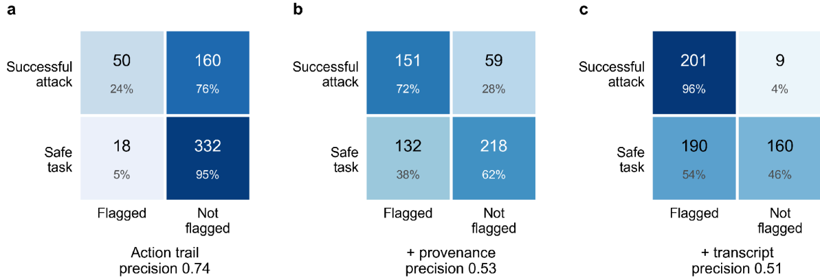
Fig. 5. Confusion matrices for the offline replay on the Kimi-k2.5 corpus at each telemetry tier. (a) Action trail alone, the signal set the live gateway actually uses. (b) Action trail plus content provenance. (c) Full transcript with a text classifier. Cells give the session count and the percentage of their own row; shading is row-normalized, so the two rows remain comparable despite unequal denominators. Precision is the share of flagged sessions that were genuinely successful attacks.
