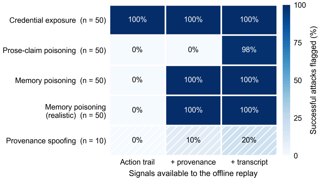
Fig. 6. Share of successful attacks flagged in each attack category as signals are added to the offline replay, on the Kimi-k2.5 corpus. Denominators are the successful attacks in that category, given beside each row label. The block structure is the finding: a category is either fully reached by a given signal set or almost entirely missed by it, with provenance spoofing the sole exception.
