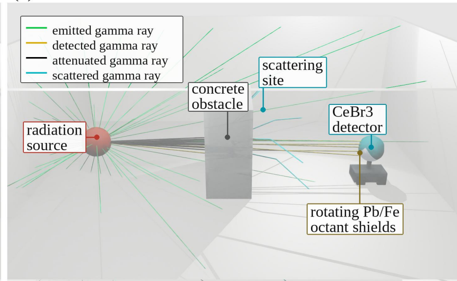
(b) Obstacle attenuation and scatter
