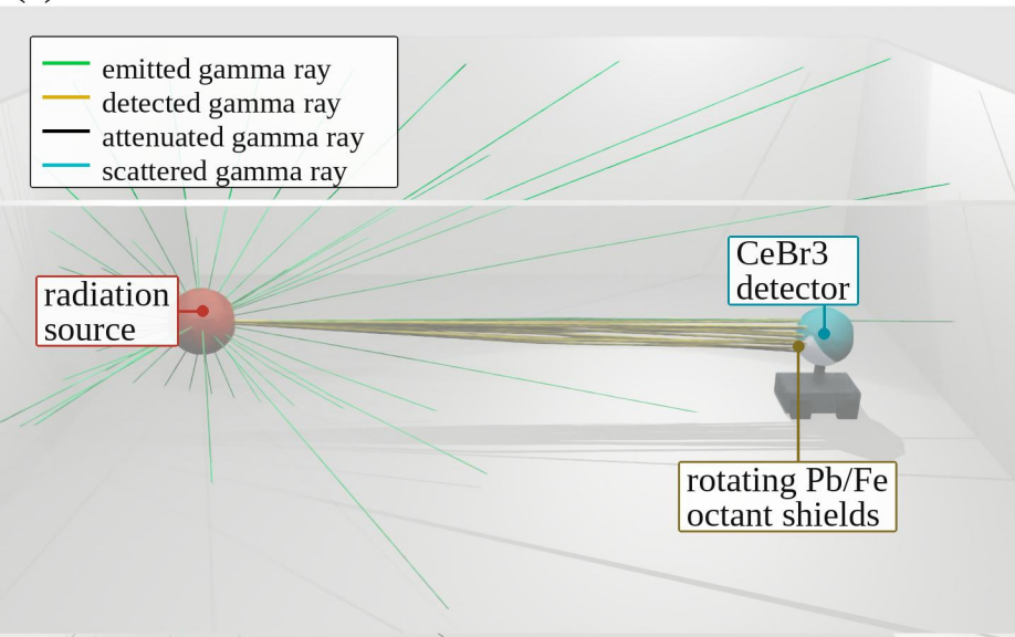
(a) Omnidirectional emission and detector hits
