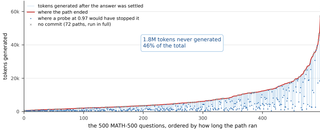
Figure 4: Where each MATH-500 path ended naturally against where a probe at 0.97 would have committed it in tokens generated (DeepSeek-R1-8B)
