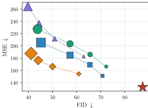
Inpainting
