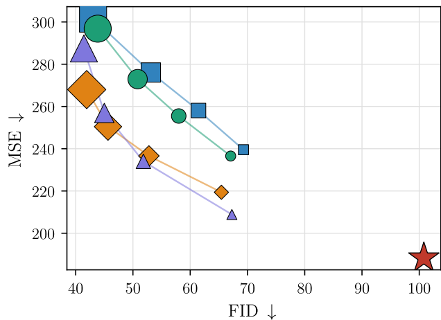
Super-resolution
