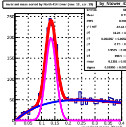
Invariant mass sorted by North 414 tower (row: 19, col: 19) by Ntower_414
