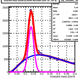
Invariant mass sorted by North 403 tower (row: 19, col: 8) by Ntower_403
