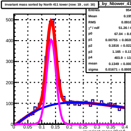
Invariant mass sorted by North 411 tower (row: 19, col: 16) by Ntower_411
