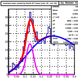
Invariant mass sorted by North 417 tower (row: 19, col: 22) by Ntower_417
