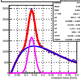
Invariant mass sorted by North 398 tower (row: 19, col: 3) by Ntower_398
