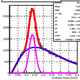
Invariant mass sorted by North 399 tower (row: 19, col: 4) by Ntower_399
