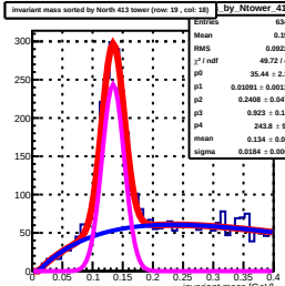
Invariant mass sorted by North 413 tower (row: 19, col: 18) by Ntower_413
