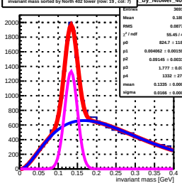
Invariant mass sorted by North 402 tower (row: 19, col: 7) by Ntower_402
