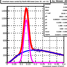
Invariant mass sorted by North 406 tower (row: 19, col: 11) by Ntower_406
