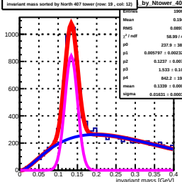
Invariant mass sorted by North 407 tower (row: 19, col: 12) by Ntower_407
