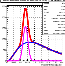
Invariant mass sorted by North 401 tower (row: 19, col: 6) by Ntower_401
