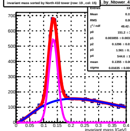
Invariant mass sorted by North 410 tower (row: 19, col: 15) by Ntower_410
