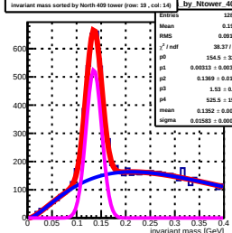
Invariant mass sorted by North 409 tower (row: 19, col: 14) by Ntower_409
