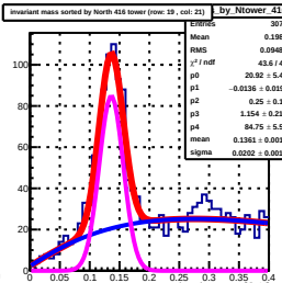
Invariant mass sorted by North 416 tower (row: 19, col: 21) by Ntower_416
