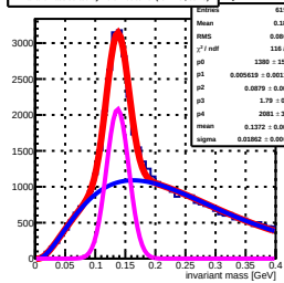
Invariant mass sorted by North 400 tower (row: 19, col: 5) by Ntower_400
