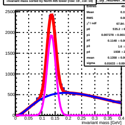
Invariant mass sorted by North 405 tower (row: 19, col: 10) by Ntower_405
