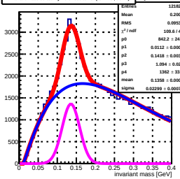
Invariant mass sorted by North 396 tower (row: 19, col: 1) by Ntower_396
