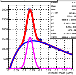
Invariant mass sorted by North 397 tower (row: 19, col: 2) by Ntower_397
