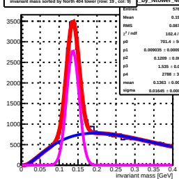
Invariant mass sorted by North 404 tower (row: 19, col: 9) by Ntower_404
