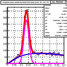
Invariant mass sorted by North 412 tower (row: 19, col: 17) by Ntower_412
