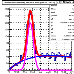
Invariant mass sorted by North 415 tower (row: 19, col: 20) by Ntower_415
