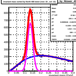
Invariant mass sorted by North 408 tower (row: 19, col: 13) by Ntower_408
