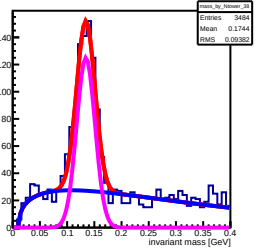
Invariant mass sorted by North 38 lower (row: 2, col: 17)
