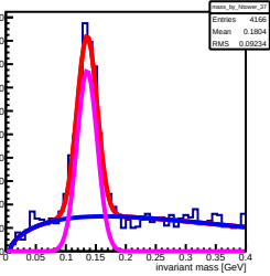
Invariant mass sorted by North 37 lower (row: 2, col: 16)
