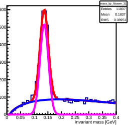
Invariant mass sorted by North 31 lower (row: 2, col: 10)
