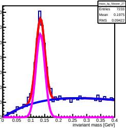
Invariant mass sorted by North 27 lower (row: 2, col: 6)
