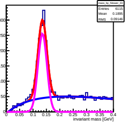
Invariant mass sorted by North 33 lower (row: 2, col: 12)
