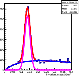
Invariant mass sorted by North 30 lower (row: 2, col: 9)
