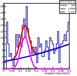
Invariant mass sorted by North 43 lower (row: 2, col: 22)
