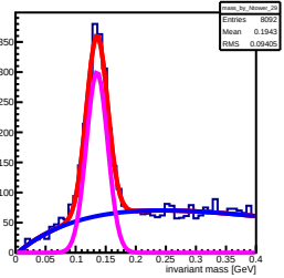
Invariant mass sorted by North 29 lower (row: 2, col: 8)
