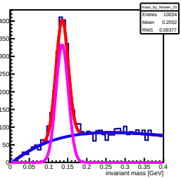
Invariant mass sorted by North 25 lower (row: 2, col: 4)
