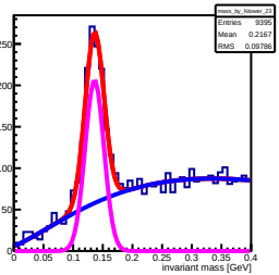
Invariant mass sorted by North 23 lower (row: 2, col: 2)
