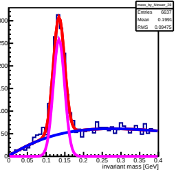
Invariant mass sorted by North 28 lower (row: 2, col: 7)
