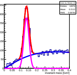
Invariant mass sorted by North 24 lower (row: 2, col: 3)
