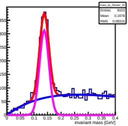
Invariant mass sorted by North 26 lower (row: 2, col: 5)
