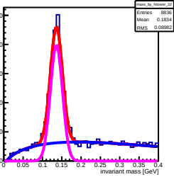
Invariant mass sorted by North 32 lower (row: 2, col: 11)
