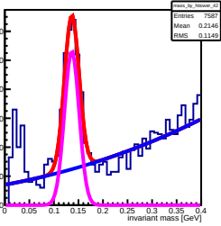
Invariant mass sorted by North 42 lower (row: 2, col: 21)
