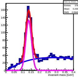
Invariant mass sorted by South 305 tower (row: 14 , col: 20)
