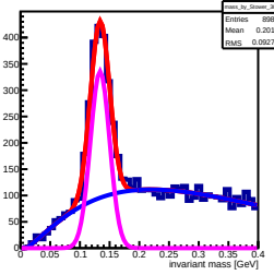
Invariant mass sorted by South 300 tower (row: 14 , col: 15)
