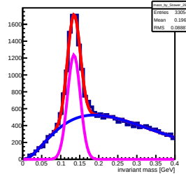
Invariant mass sorted by South 294 tower (row: 14 , col: 9)
