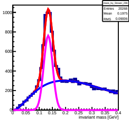
Invariant mass sorted by South 296 tower (row: 14 , col: 11)
