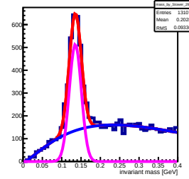
Invariant mass sorted by South 299 tower (row: 14 , col: 14)
