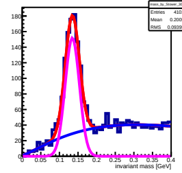
Invariant mass sorted by South 304 tower (row: 14 , col: 19)
