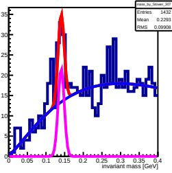
Invariant mass sorted by South 307 tower (row: 14 , col: 22)
