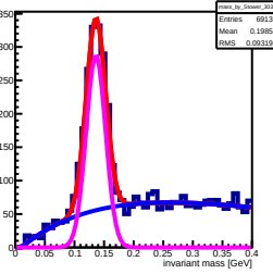
Invariant mass sorted by South 303 tower (row: 14 , col: 18)
