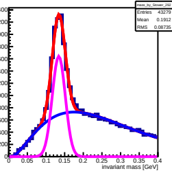
Invariant mass sorted by South 292 tower (row: 14 , col: 7)
