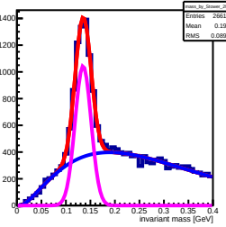
Invariant mass sorted by South 295 tower (row: 14 , col: 10)
