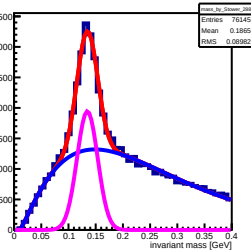
Invariant mass sorted by South 288 tower (row: 14 , col: 3)
