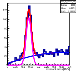
Invariant mass sorted by South 306 tower (row: 14 , col: 21)
