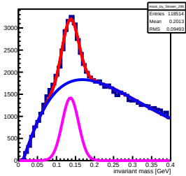
Invariant mass sorted by South 286 tower (row: 14 , col: 1)
