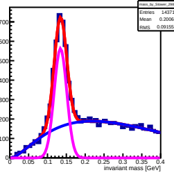
Invariant mass sorted by South 298 tower (row: 14 , col: 13)
