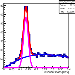
Invariant mass sorted by South 302 tower (row: 14 , col: 17)
