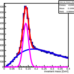
Invariant mass sorted by South 293 tower (row: 14 , col: 8)
