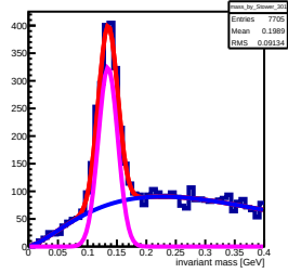
Invariant mass sorted by South 301 tower (row: 14 , col: 16)
