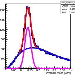
Invariant mass sorted by South 290 tower (row: 14 , col: 5)
