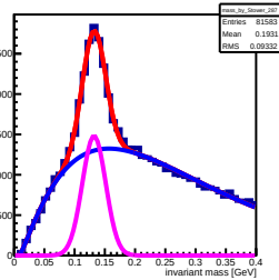
Invariant mass sorted by South 287 tower (row: 14 , col: 2)
