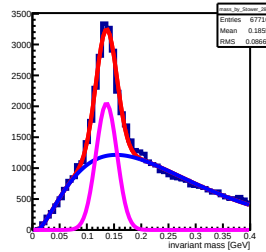
Invariant mass sorted by South 289 tower (row: 14 , col: 4)
