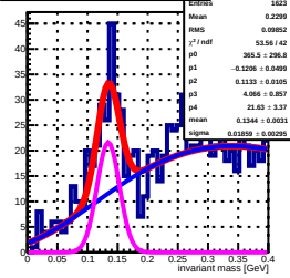
invariant mass sorted by South 373 tower (row: 17, col: 22) by Stower 373
