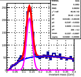
invariant mass sorted by South 369 tower (row: 17, col: 18) by Stower 369
