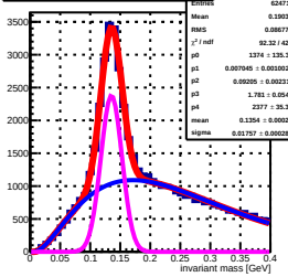
invariant mass sorted by South 357 tower (row: 17, col: 6) by Stower 357
