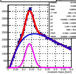
invariant mass sorted by South 352 tower (row: 17, col: 1) by Stower 352
