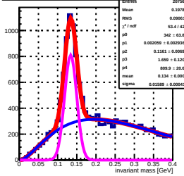
invariant mass sorted by South 362 tower (row: 17, col: 11) by Stower 362
