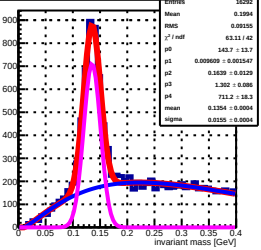
invariant mass sorted by South 365 tower (row: 17, col: 14) by Stower 365
