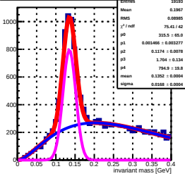
invariant mass sorted by South 363 tower (row: 17, col: 12) by Stower 363
