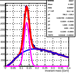
invariant mass sorted by South 360 tower (row: 17, col: 9) by Stower 360
