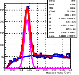
invariant mass sorted by South 371 tower (row: 17, col: 20) by Stower 371
