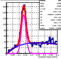
invariant mass sorted by South 372 tower (row: 17, col: 21) by Stower 372
