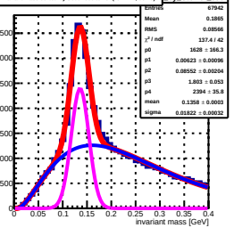
invariant mass sorted by South 352 tower (row: 17, col: 5) by Stower 352
