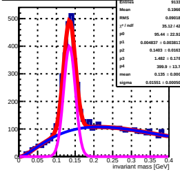
invariant mass sorted by South 367 tower (row: 17, col: 16) by Stower 367
