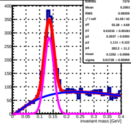
invariant mass sorted by South 368 tower (row: 17, col: 17) by Stower 368
