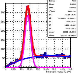
invariant mass sorted by South 370 tower (row: 17, col: 19) by Stower 370
