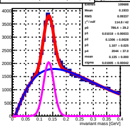
invariant mass sorted by South 352 tower (row: 17, col: 2) by Stower 352
