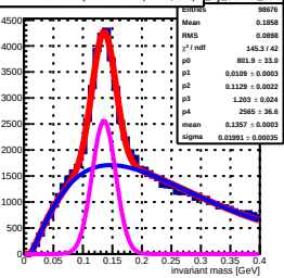
invariant mass sorted by South 352 tower (row: 17, col: 3) by Stower 352
