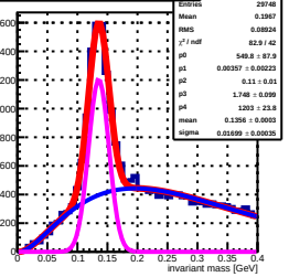
invariant mass sorted by South 361 tower (row: 17, col: 10) by Stower 361
