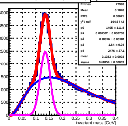
invariant mass sorted by South 352 tower (row: 17, col: 4) by Stower 352
