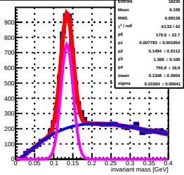
invariant mass sorted by South 364 tower (row: 17, col: 13) by Stower 364
