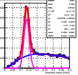
invariant mass sorted by South 366 tower (row: 17, col: 15) by Stower 366
