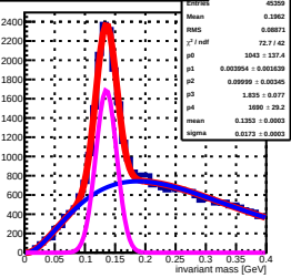
invariant mass sorted by South 359 tower (row: 17, col: 8) by Stower 359
