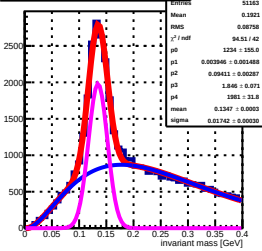
invariant mass sorted by South 358 tower (row: 17, col: 7) by Stower 358
