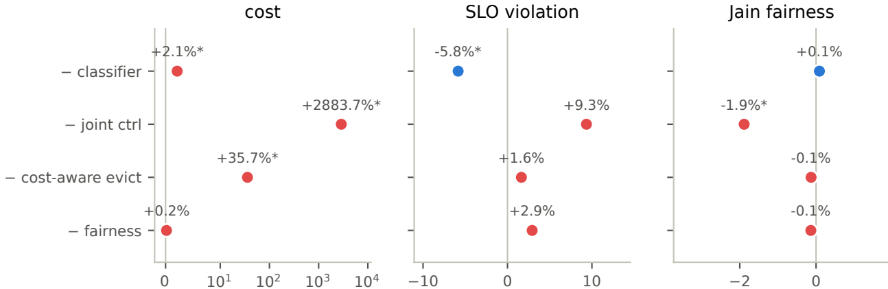
change vs full PolyForge when one component is removed (%)
