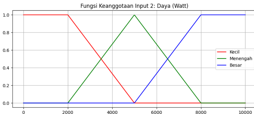
Figure 2: Membership Function Input 2: Daya Terpasang
