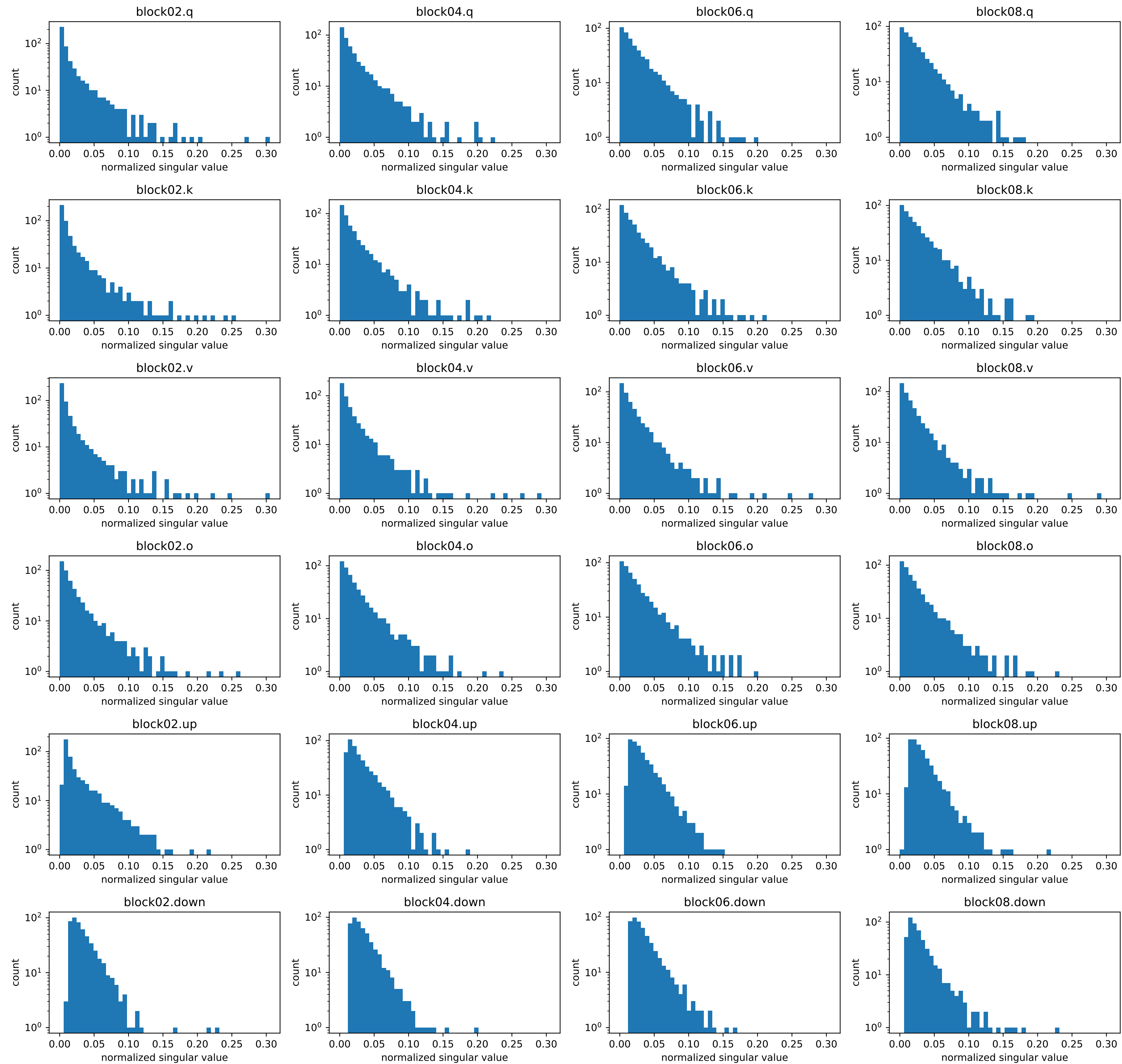
AdamW adaptive update step 1469: bulk spectrum (common bins; no bulk renormalization)
