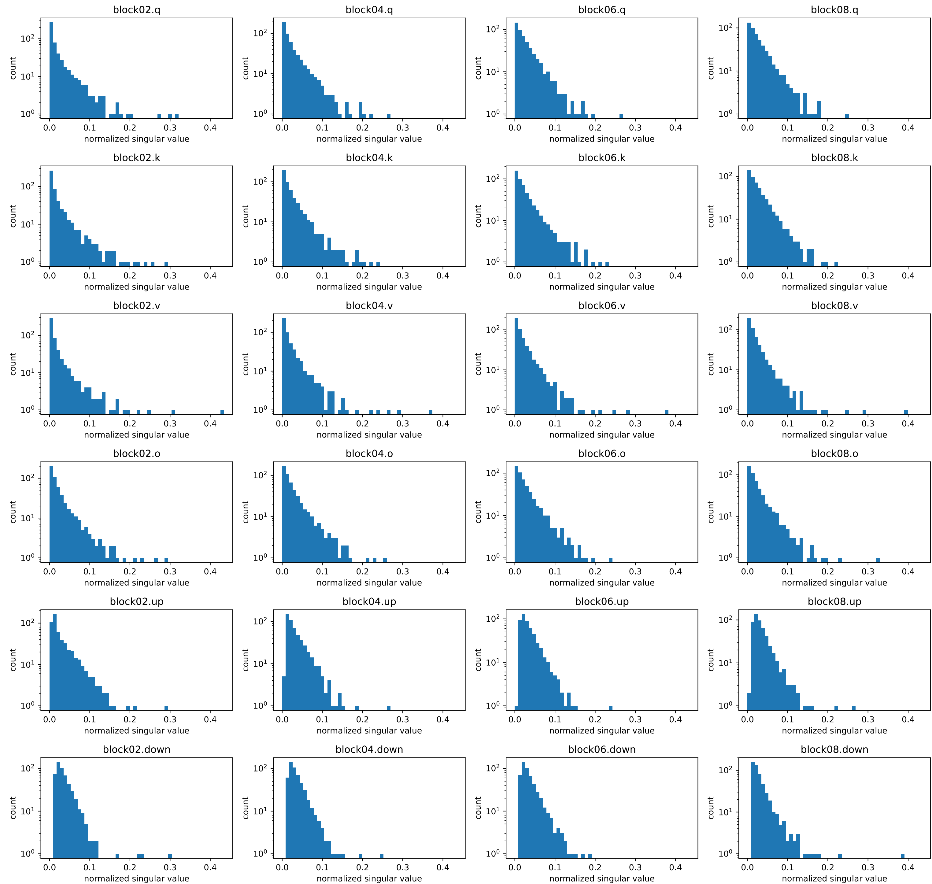
AdamW adaptive update step 1469: full spectrum (common bins; no bulk renormalization)
