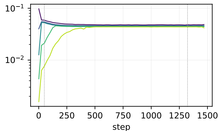
block04.o
