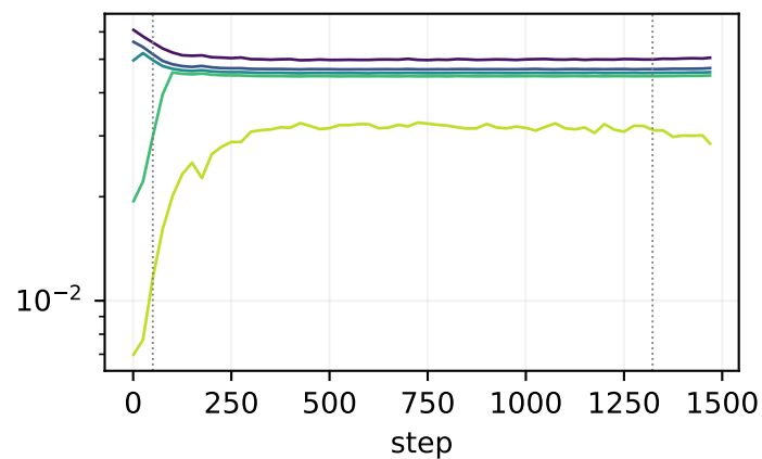
block02.v
