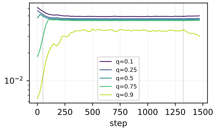
block02.k
