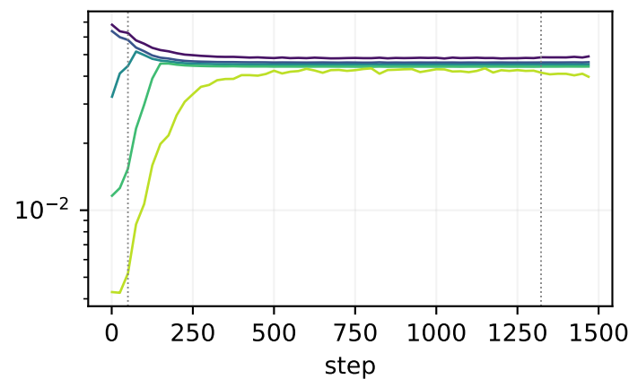
block04.v
