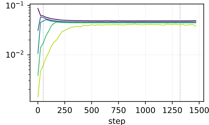
block06.o
