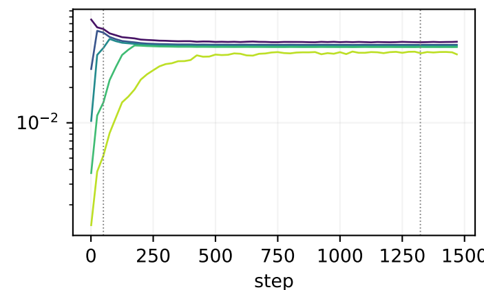
block08.o
