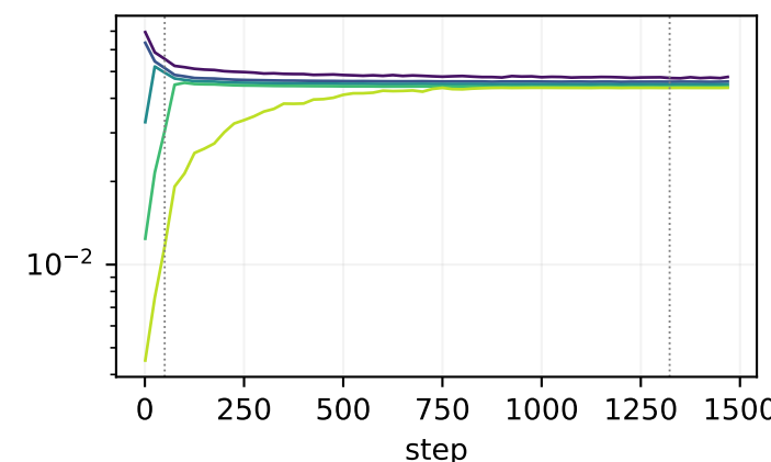
block08.up
