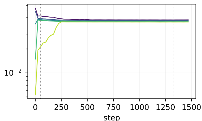
block02.up
