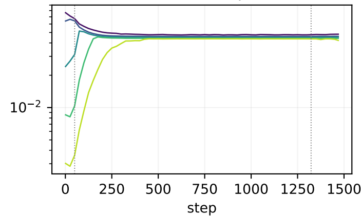
block06.k
