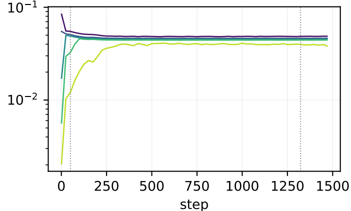
block02.o
