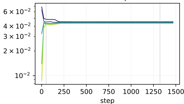
block06.down
