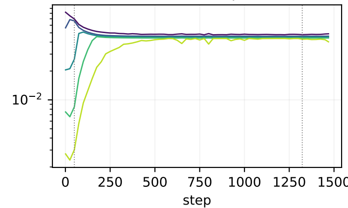
block08.k
