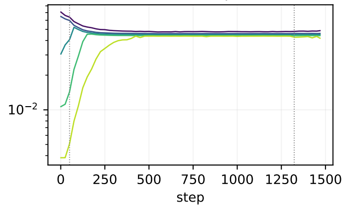
block04.k
