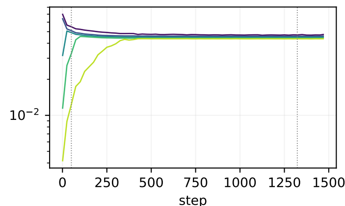
block06.up
