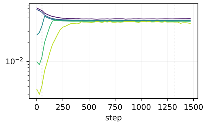
block06.v
