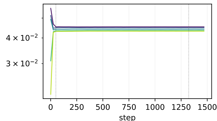
block04.down
