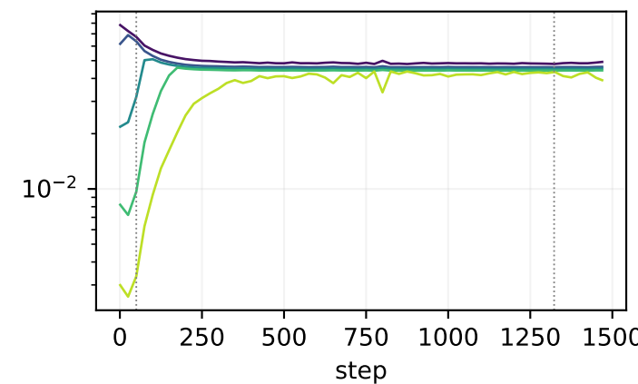
block08.v
