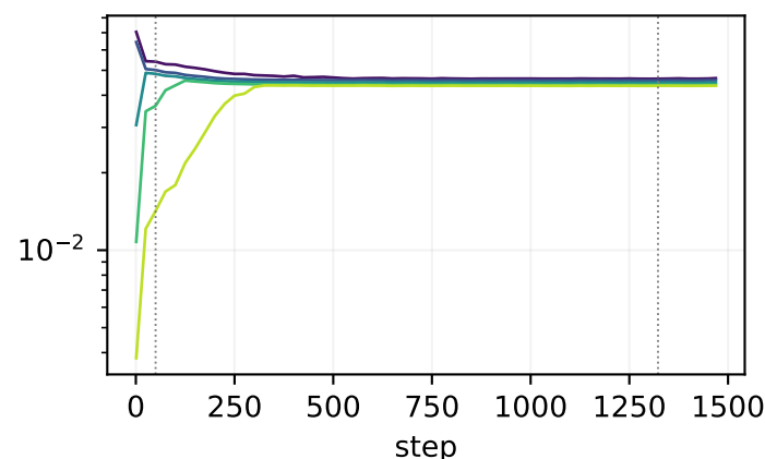
block04.up
