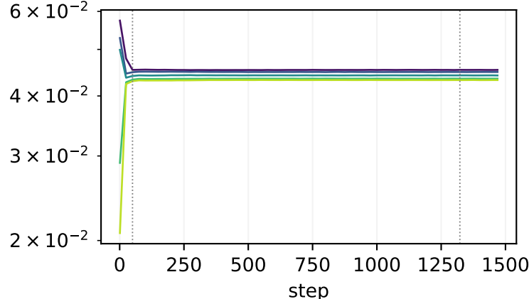
block06.down
