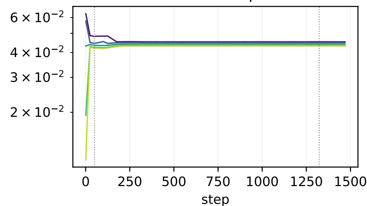
block04.down
