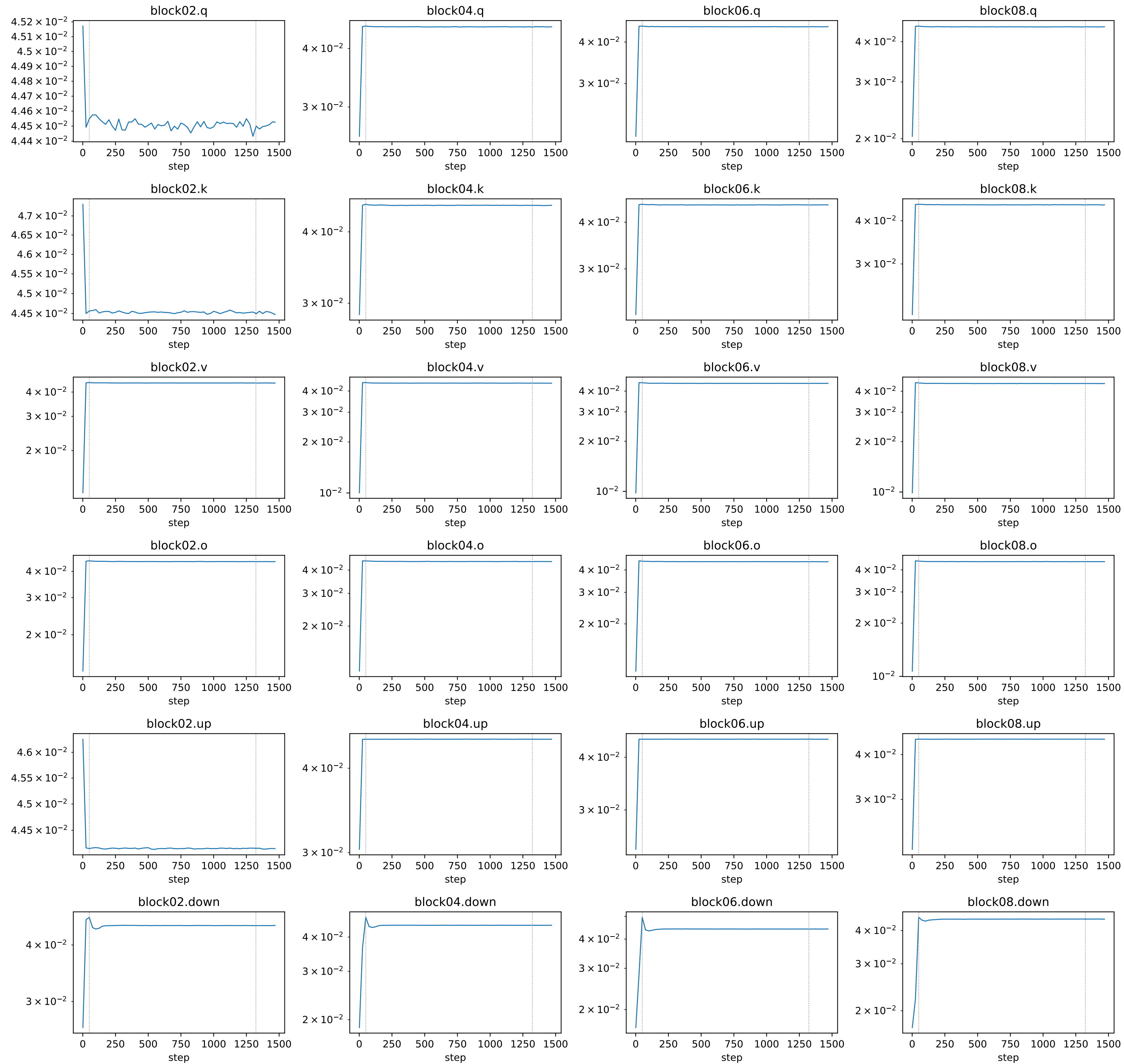
Muon post-NS update: median singular value
