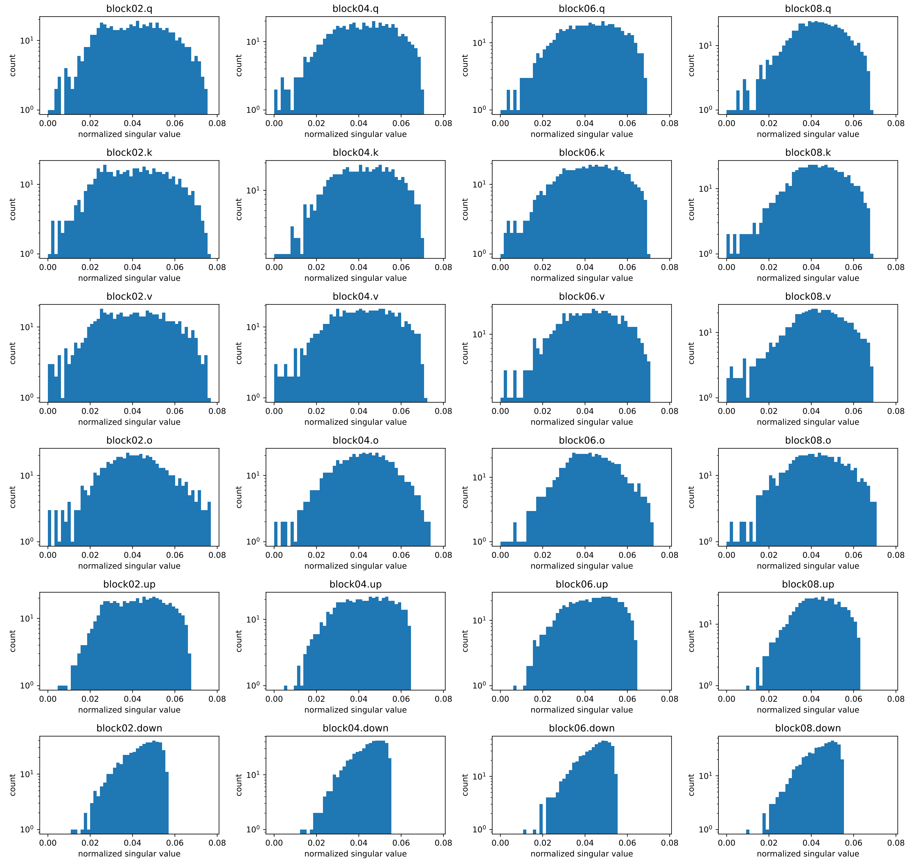
Muon post-NS update step 1028: bulk spectrum (common bins; no bulk renormalization)
