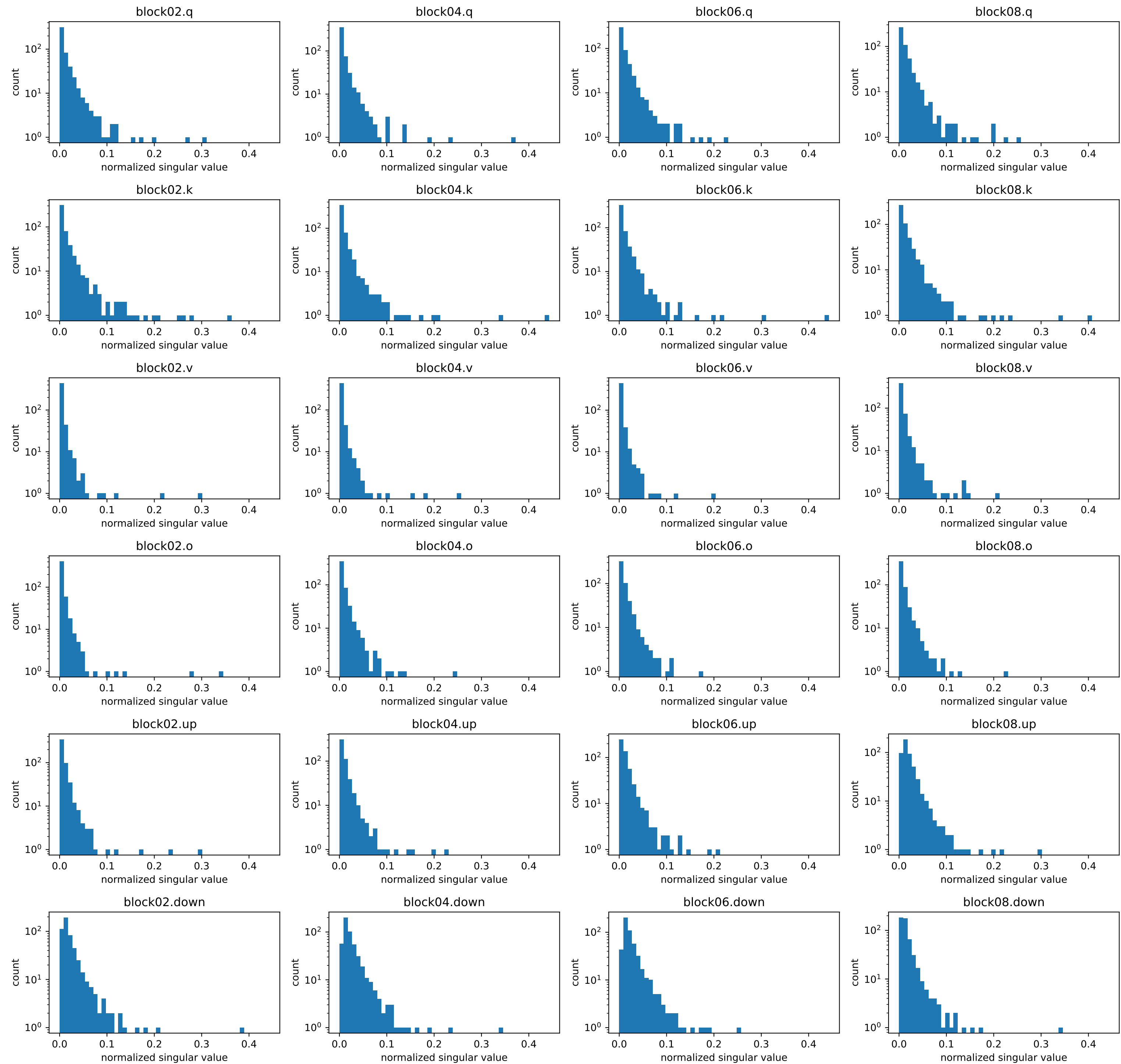
Muon pre-NS momentum step 1028: bulk spectrum (common bins; no bulk renormalization)
