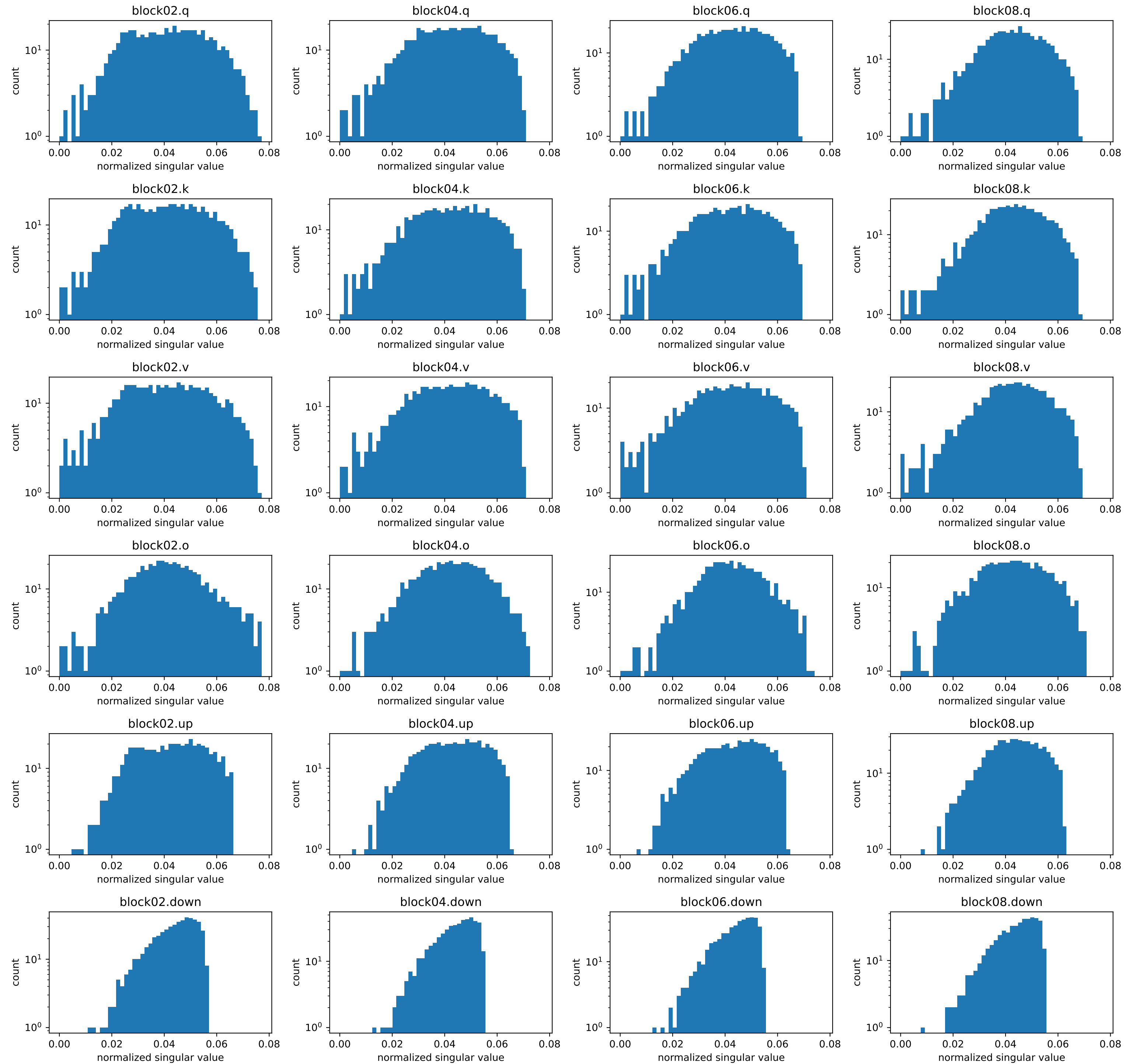
Muon post-NS update step 1249: bulk spectrum (common bins; no bulk renormalization)
