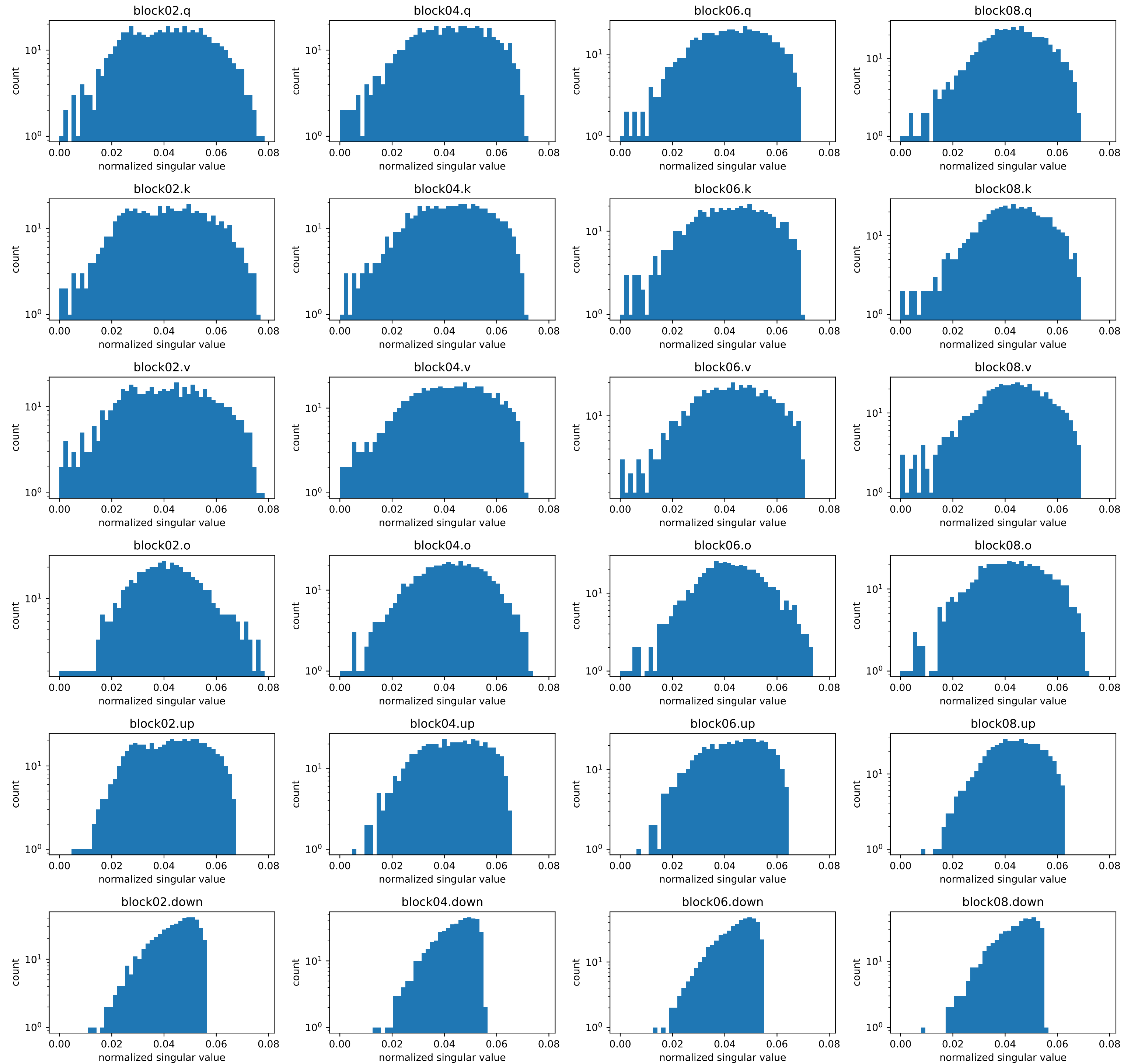
Muon post-NS update step 1249: full spectrum (common bins; no bulk renormalization)
