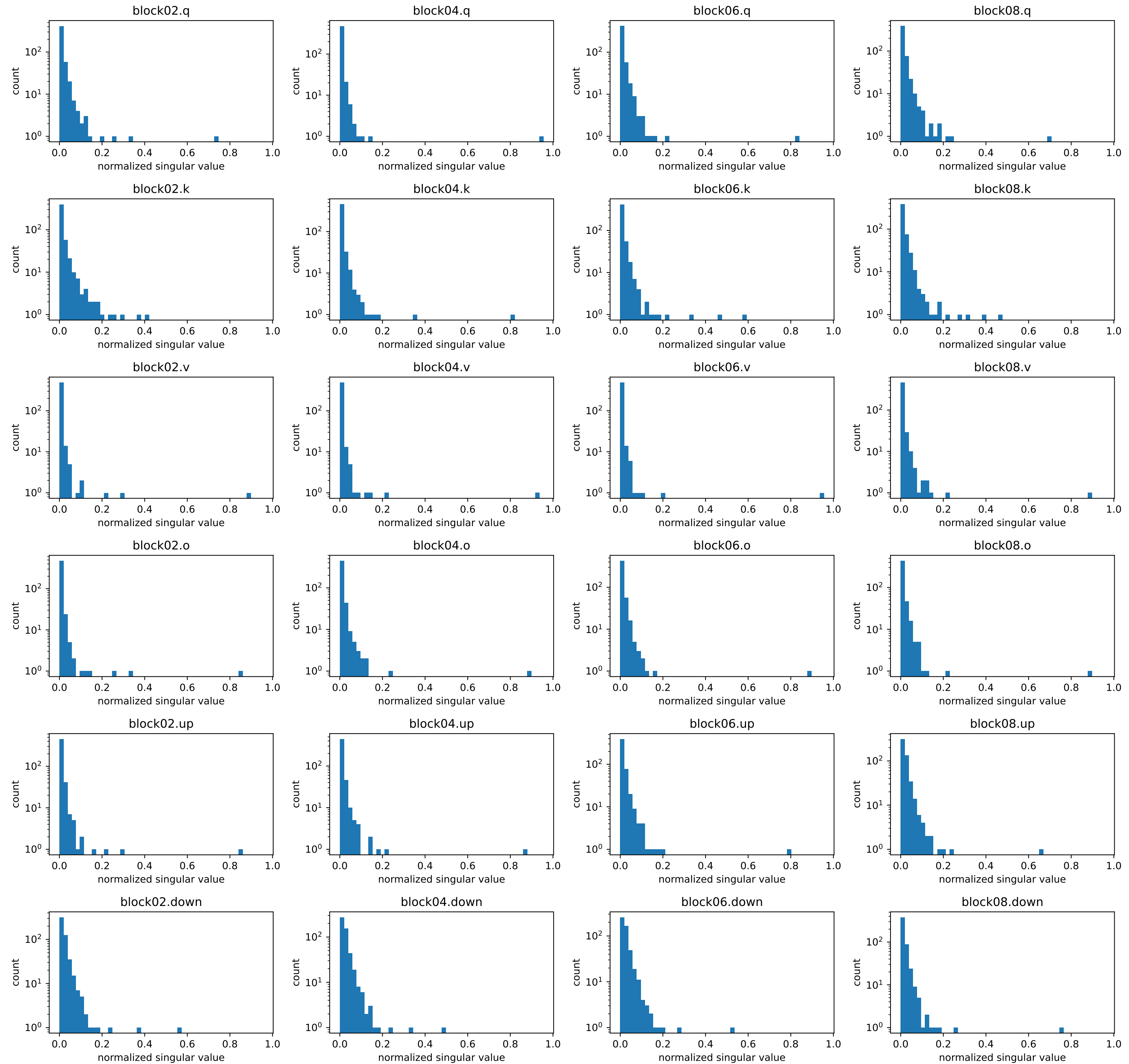
Muon pre-NS momentum step 1249: full spectrum (common bins; no bulk renormalization)
