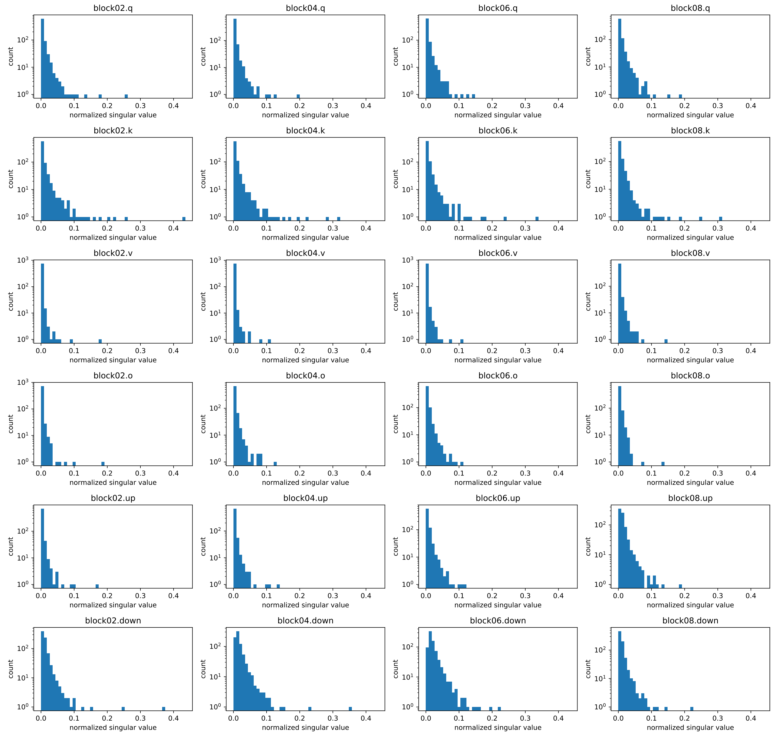
Muon pre-NS momentum step 2562: bulk spectrum (common bins; no bulk renormalization)
