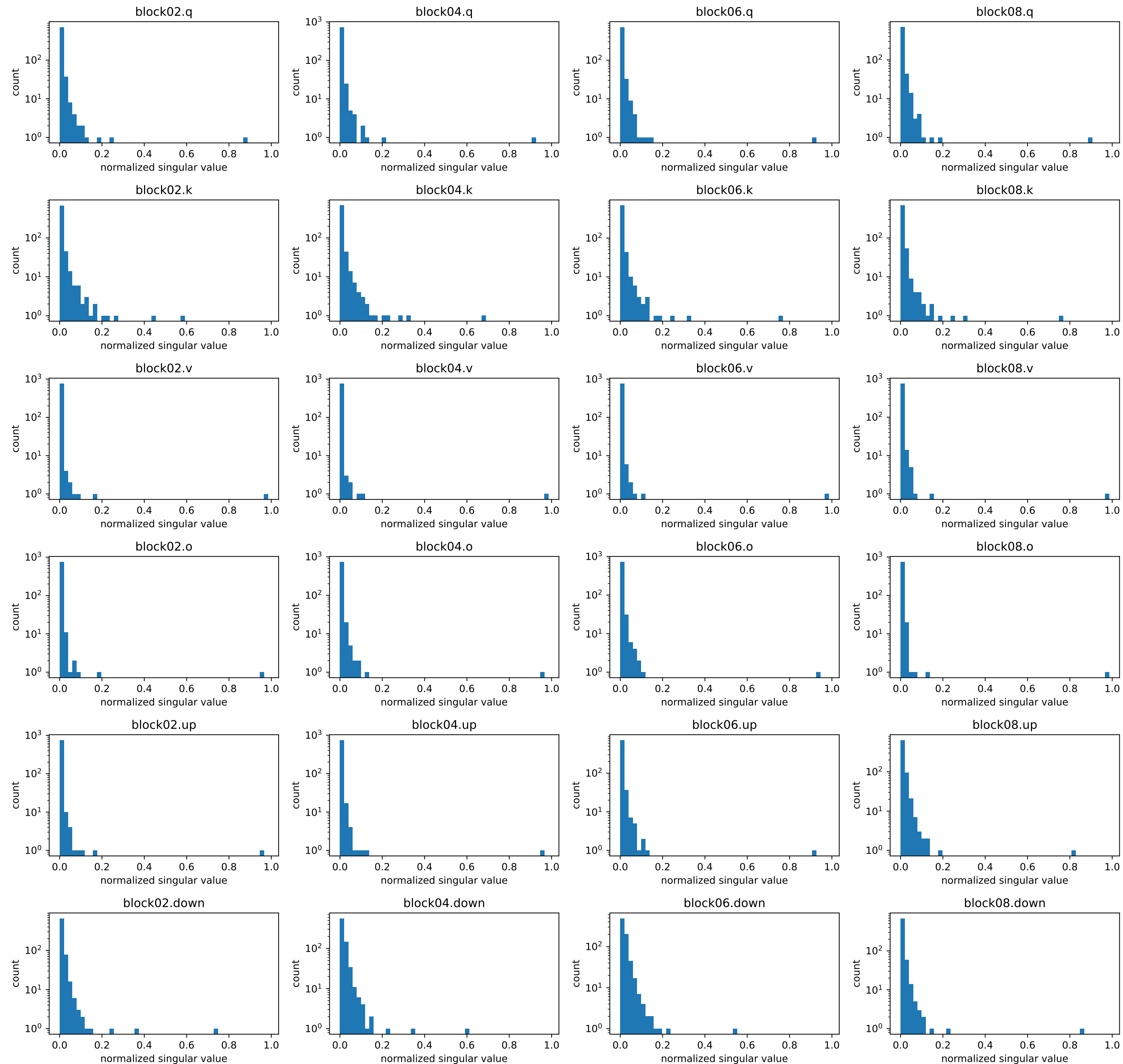
Muon pre-NS momentum step 2562: full spectrum (common bins; no bulk renormalization)
