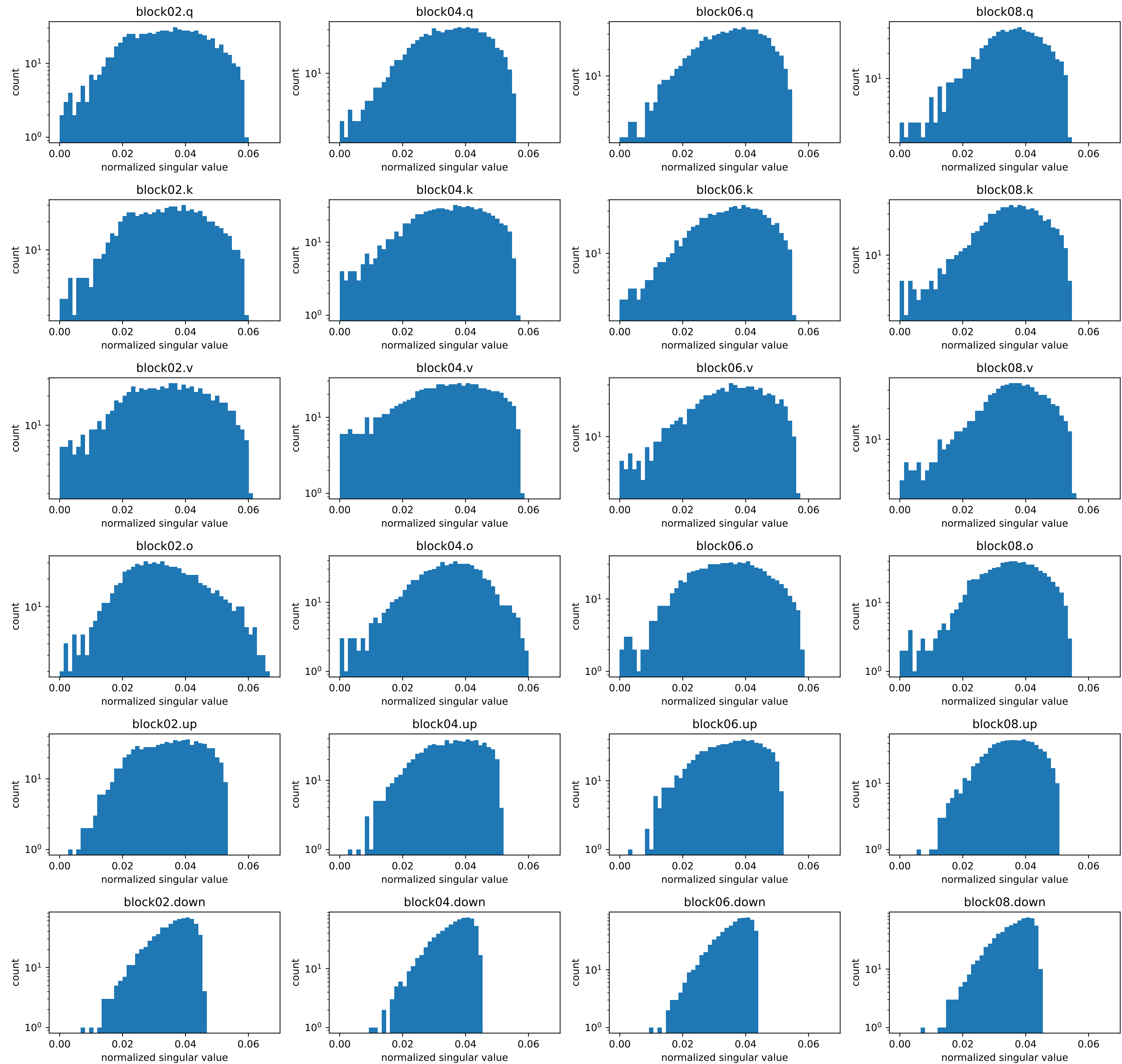
Muon post-NS update step 2562: bulk spectrum (common bins; no bulk renormalization)
