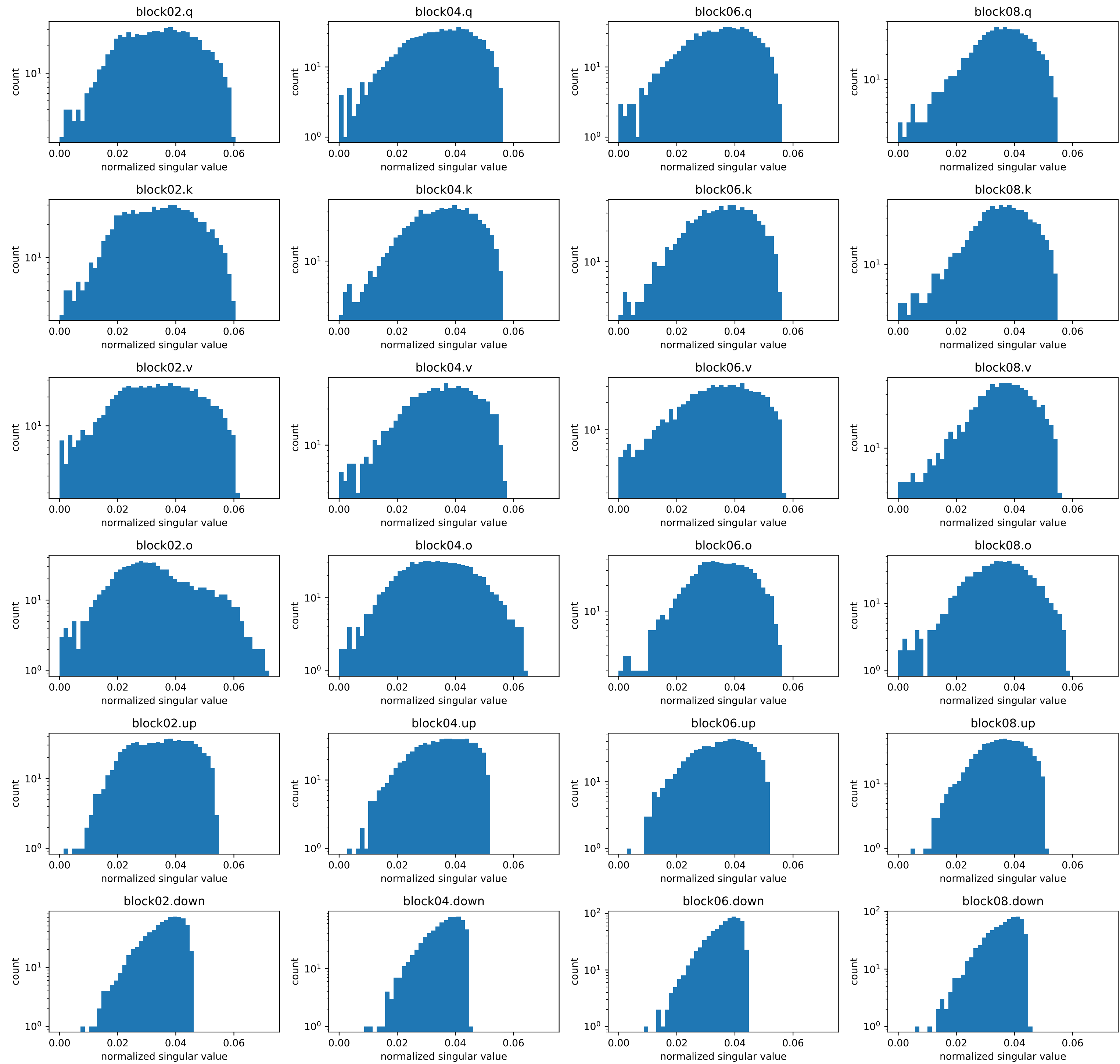
Muon post-NS update step 2562: full spectrum (common bins; no bulk renormalization)
