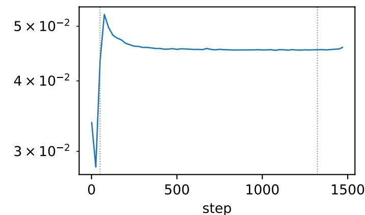
block06.o
