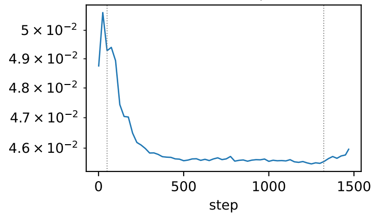
block02.k
