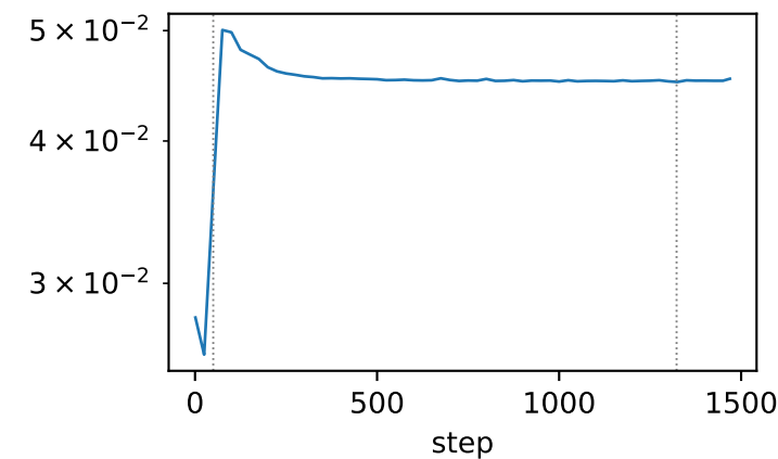
block06.v
