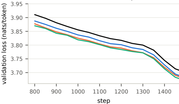
(a) validation loss, last 700 steps (one seed)
