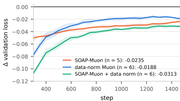
(b) difference from tuned Muon (all seeds)
