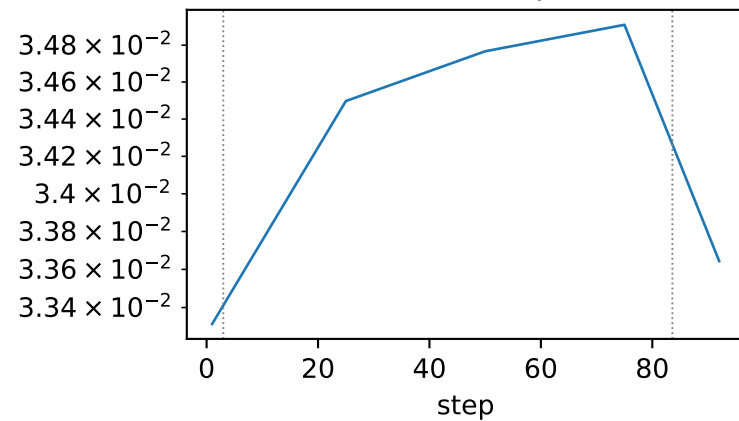
block02.k
