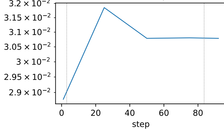
block08.k
