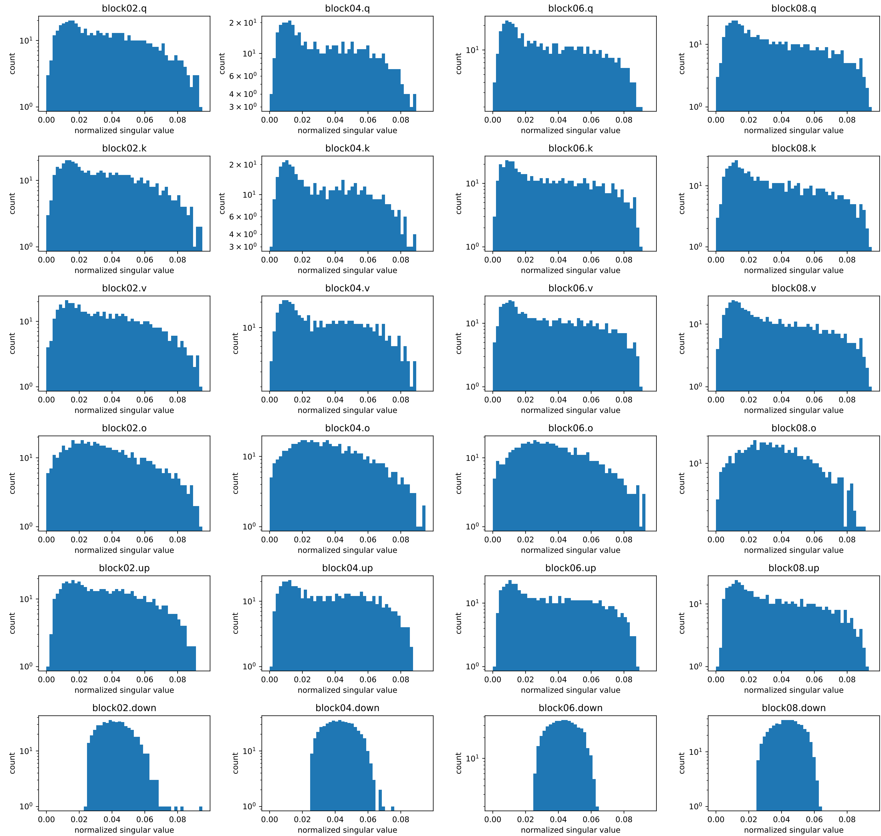
Muon post-NS update step 92: full spectrum (common bins; no bulk renormalization)
