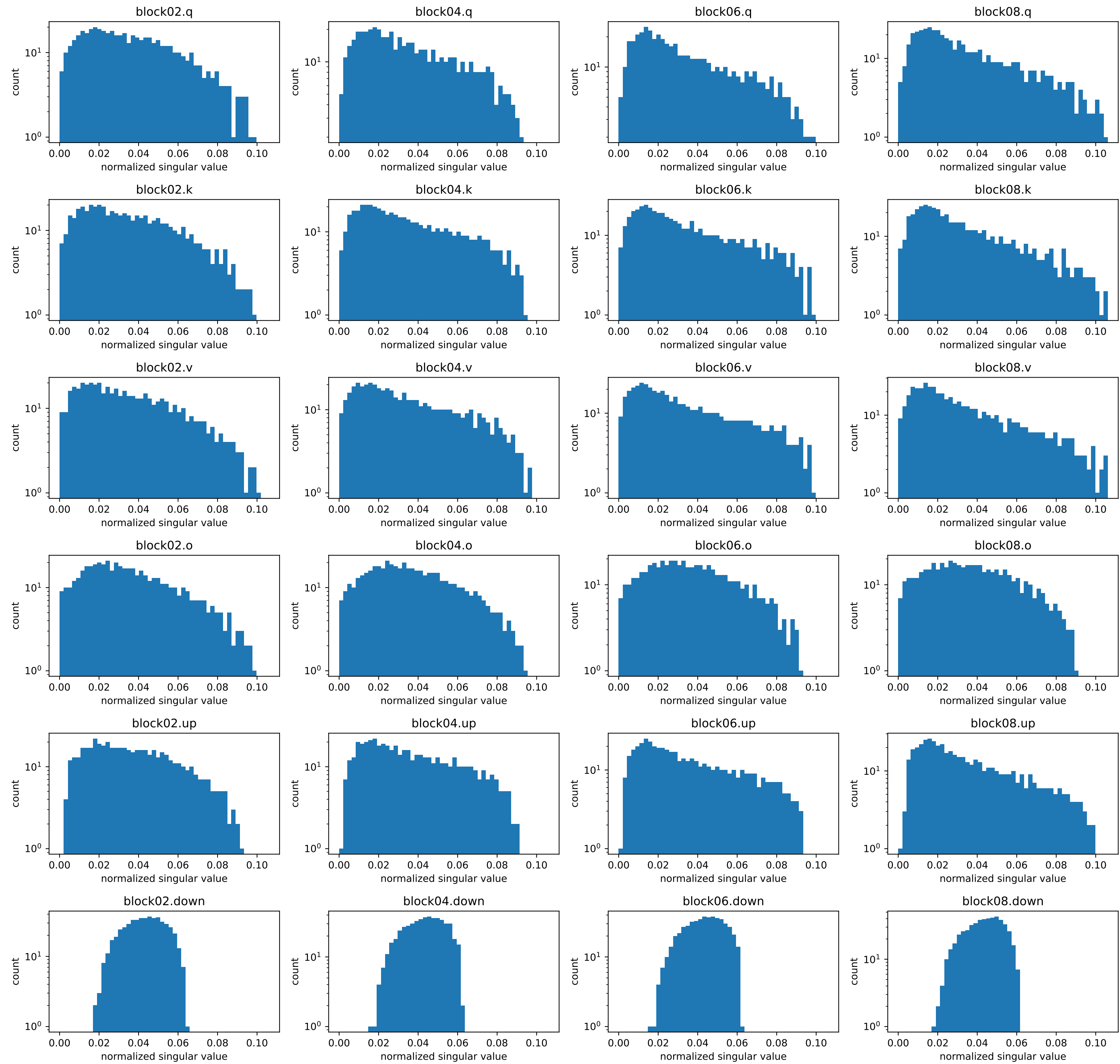
Muon post-NS update step 92: bulk spectrum (common bins; no bulk renormalization)
