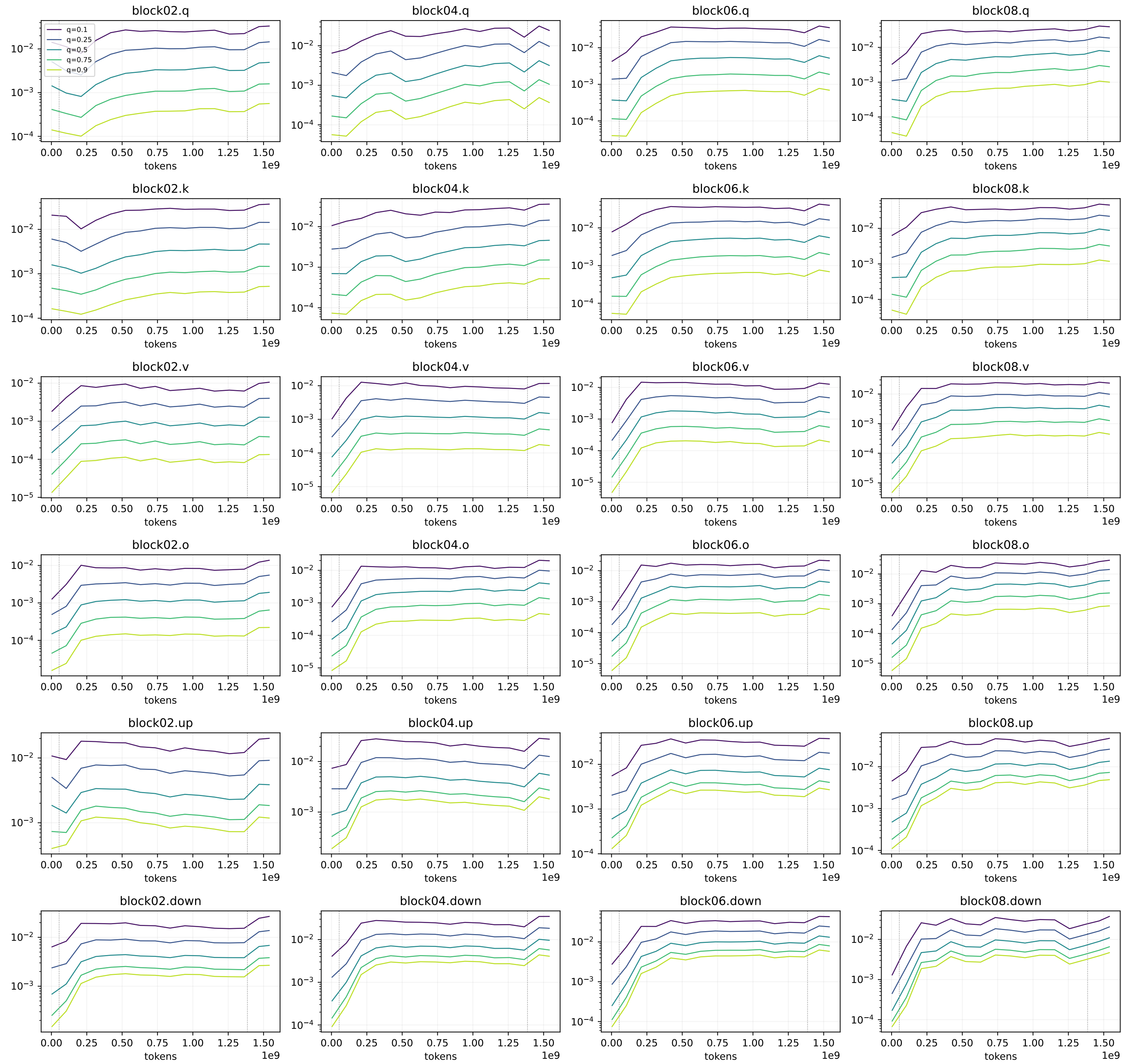
Muon pre-NS momentum: normalized descending-rank quantiles
