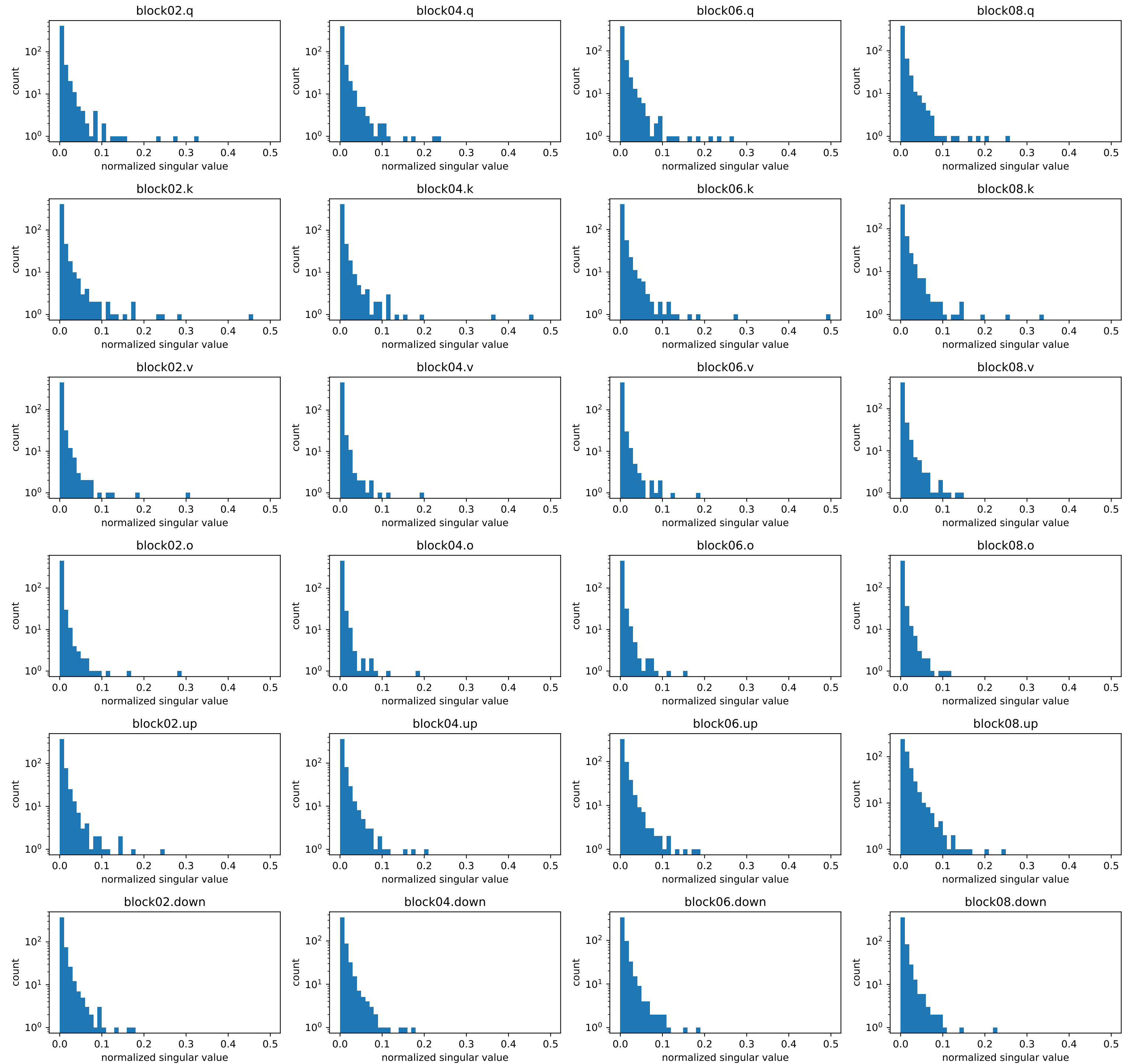
Muon pre-NS momentum step 92: bulk spectrum (common bins; no bulk renormalization)
