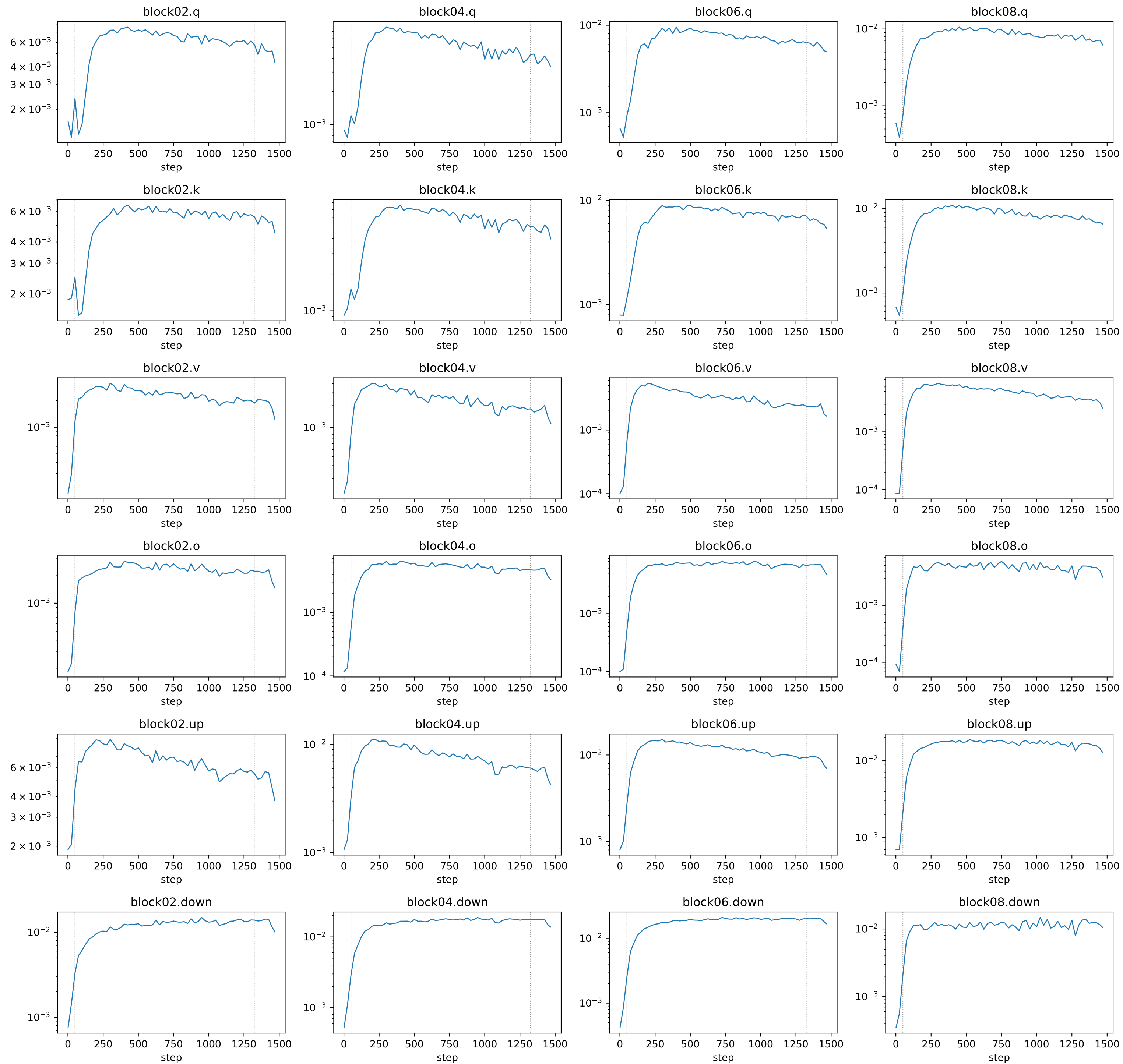
Muon pre-NS momentum: median singular value
