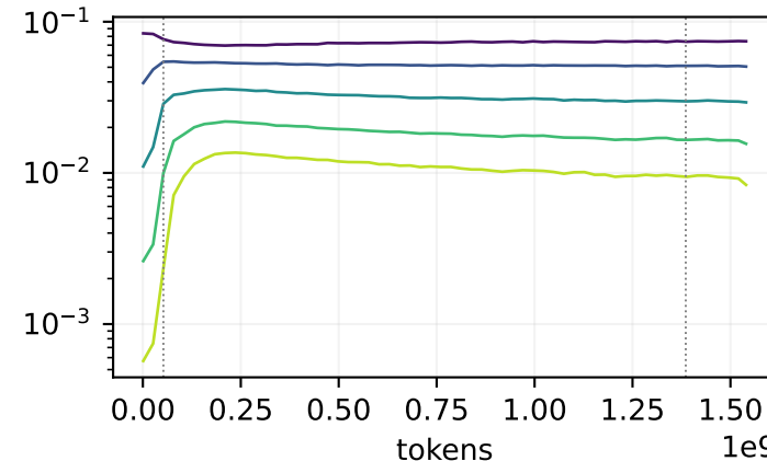
block06.o
