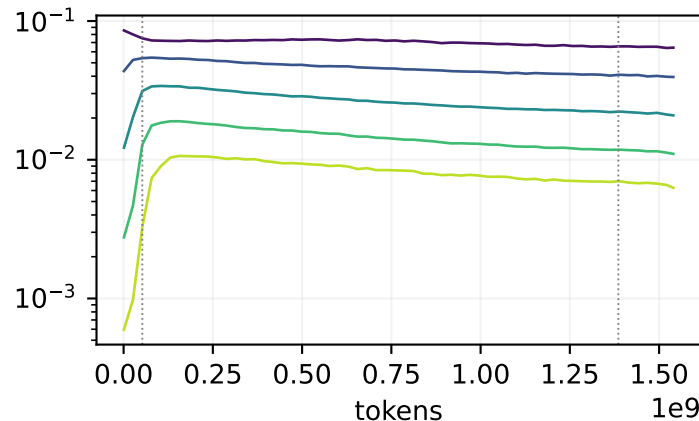
block02.o
