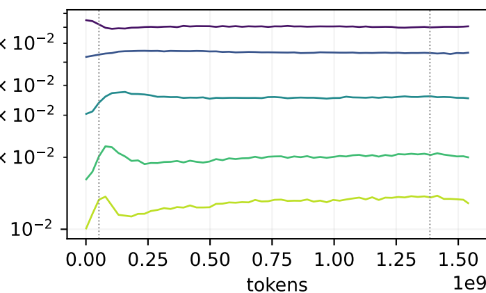
block02.down
