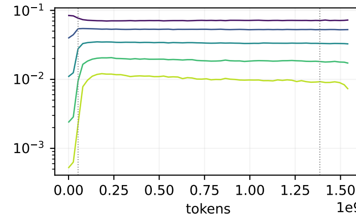
block08.o
