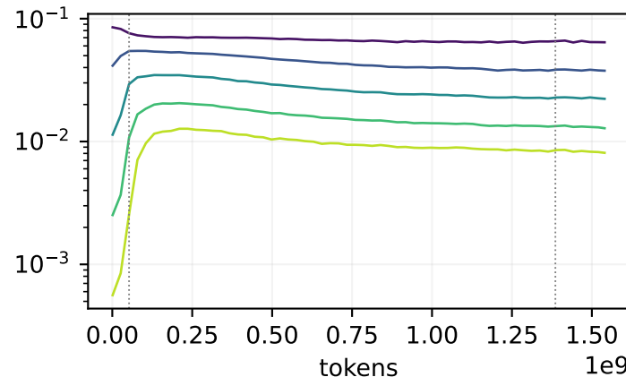
block04.o
