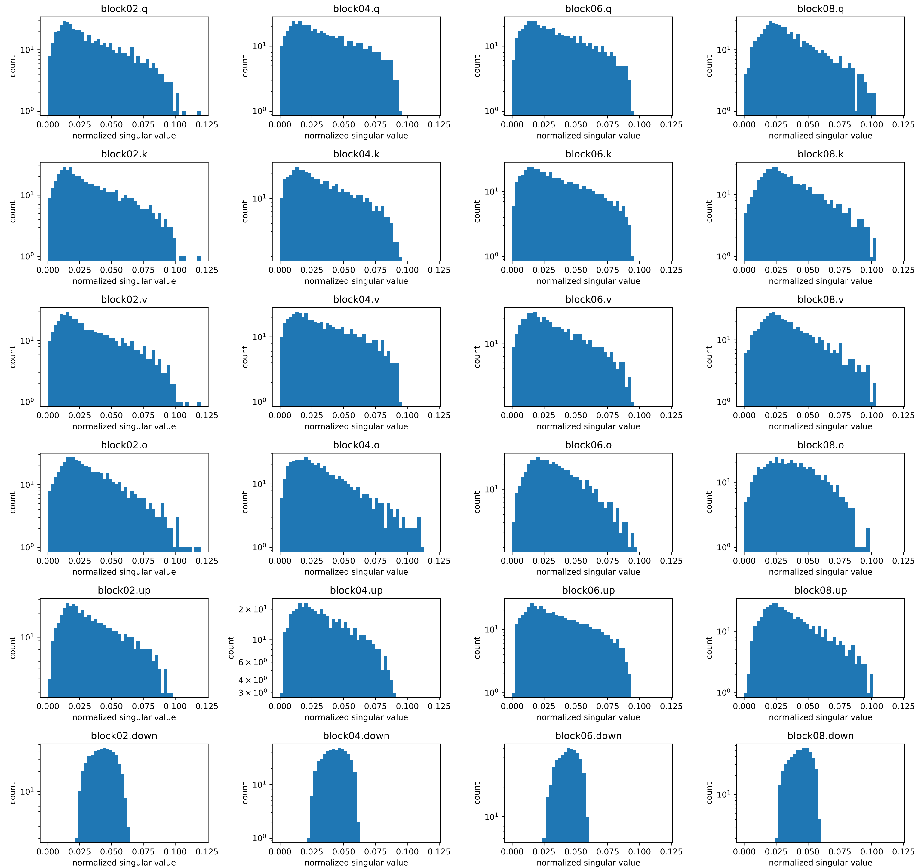
Muon post-NS update step 368: bulk spectrum (common bins; no bulk renormalization)
