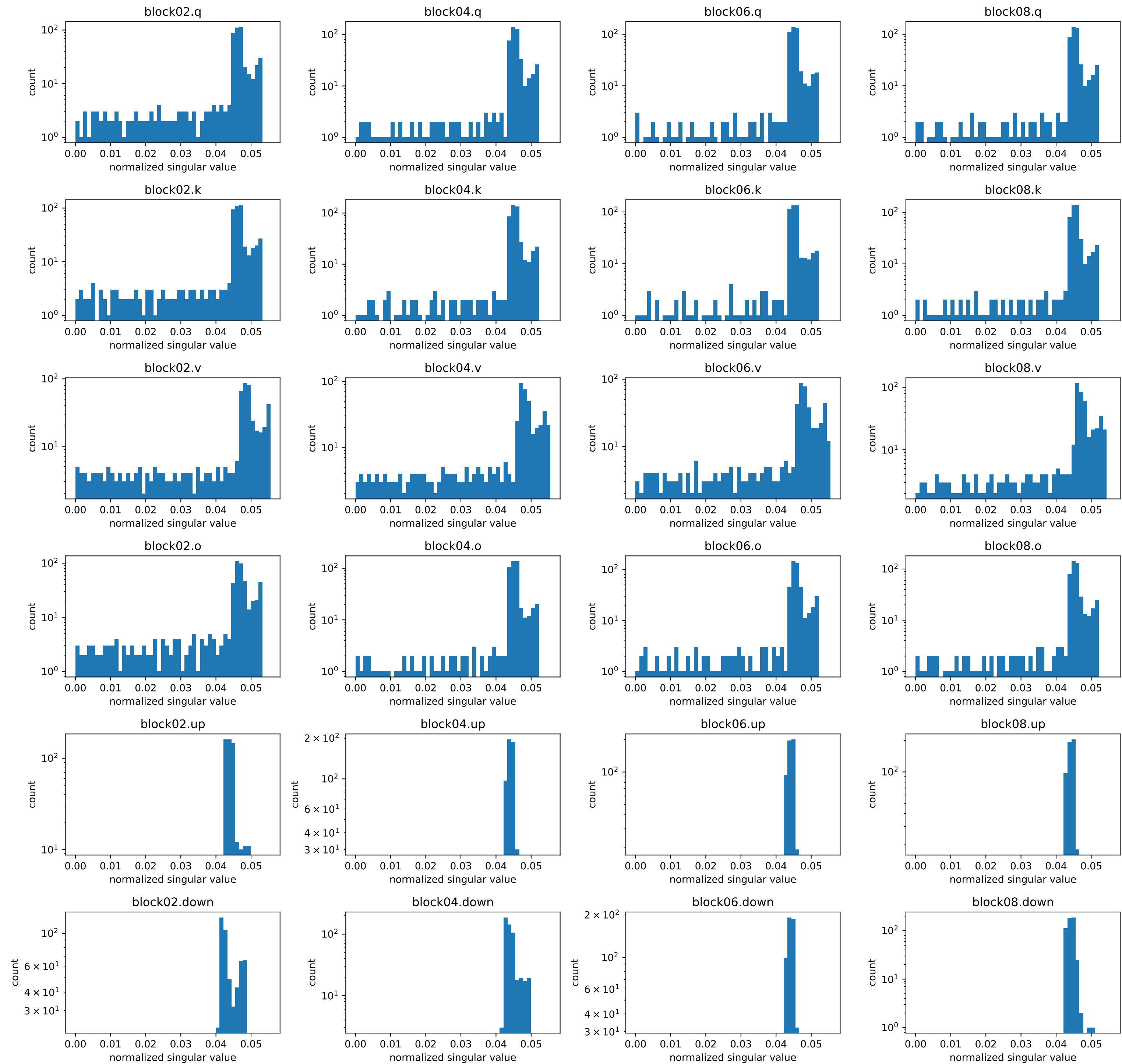
Muon post-NS update step 2938: bulk spectrum (common bins; no bulk renormalization)
