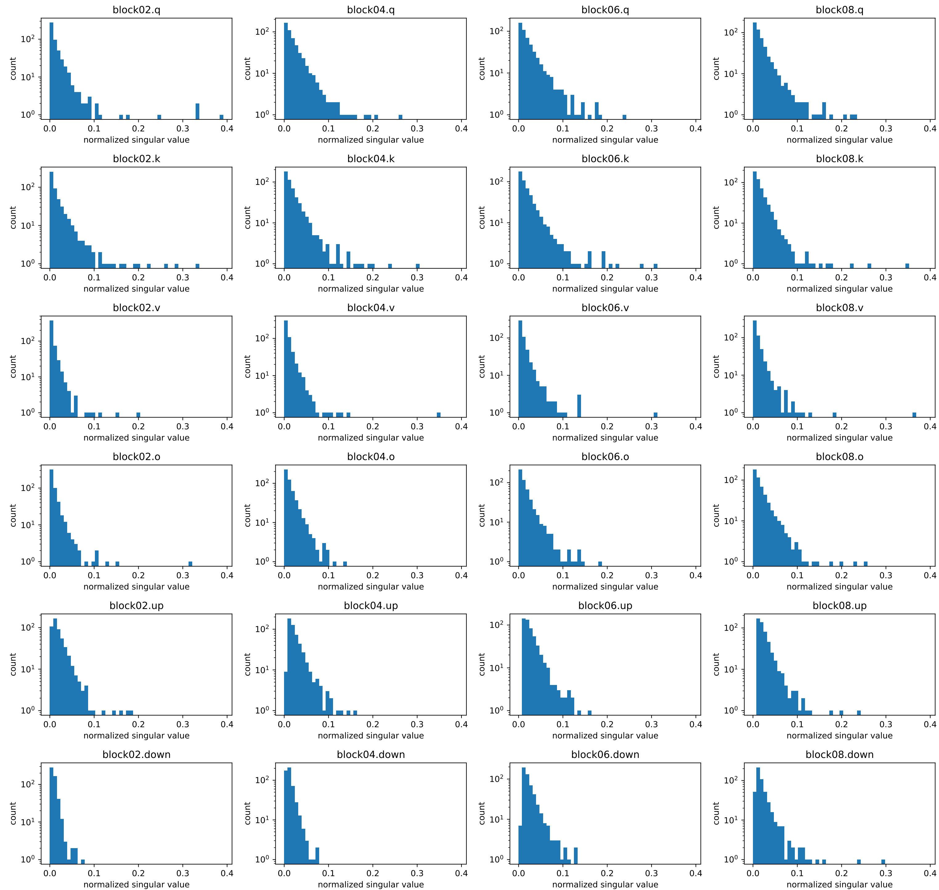
Muon pre-NS momentum step 2938: bulk spectrum (common bins; no bulk renormalization)
