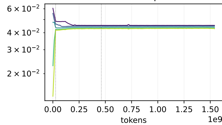
block02.down
