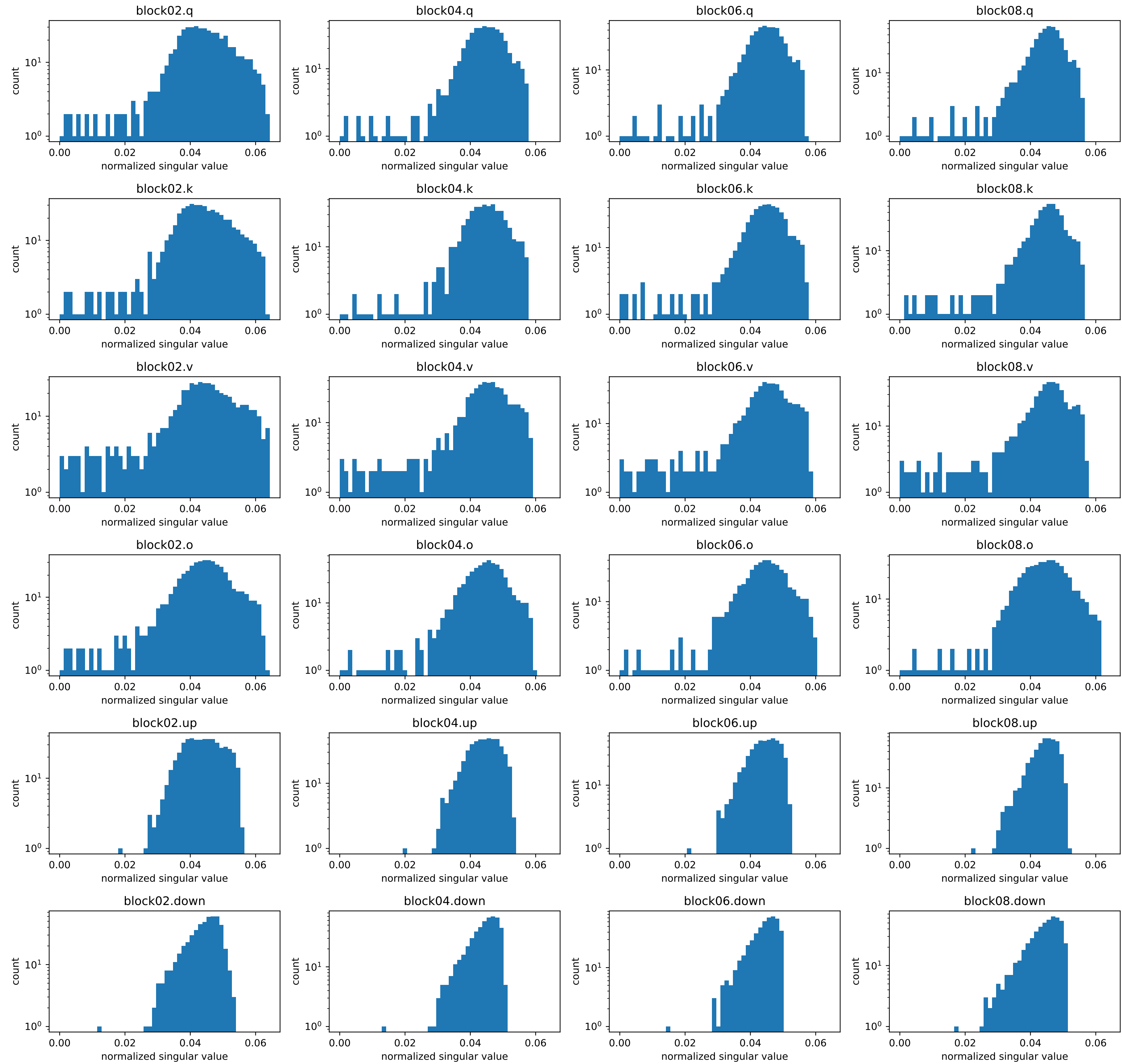
Muon post-NS update step 2938: full spectrum (common bins; no bulk renormalization)
